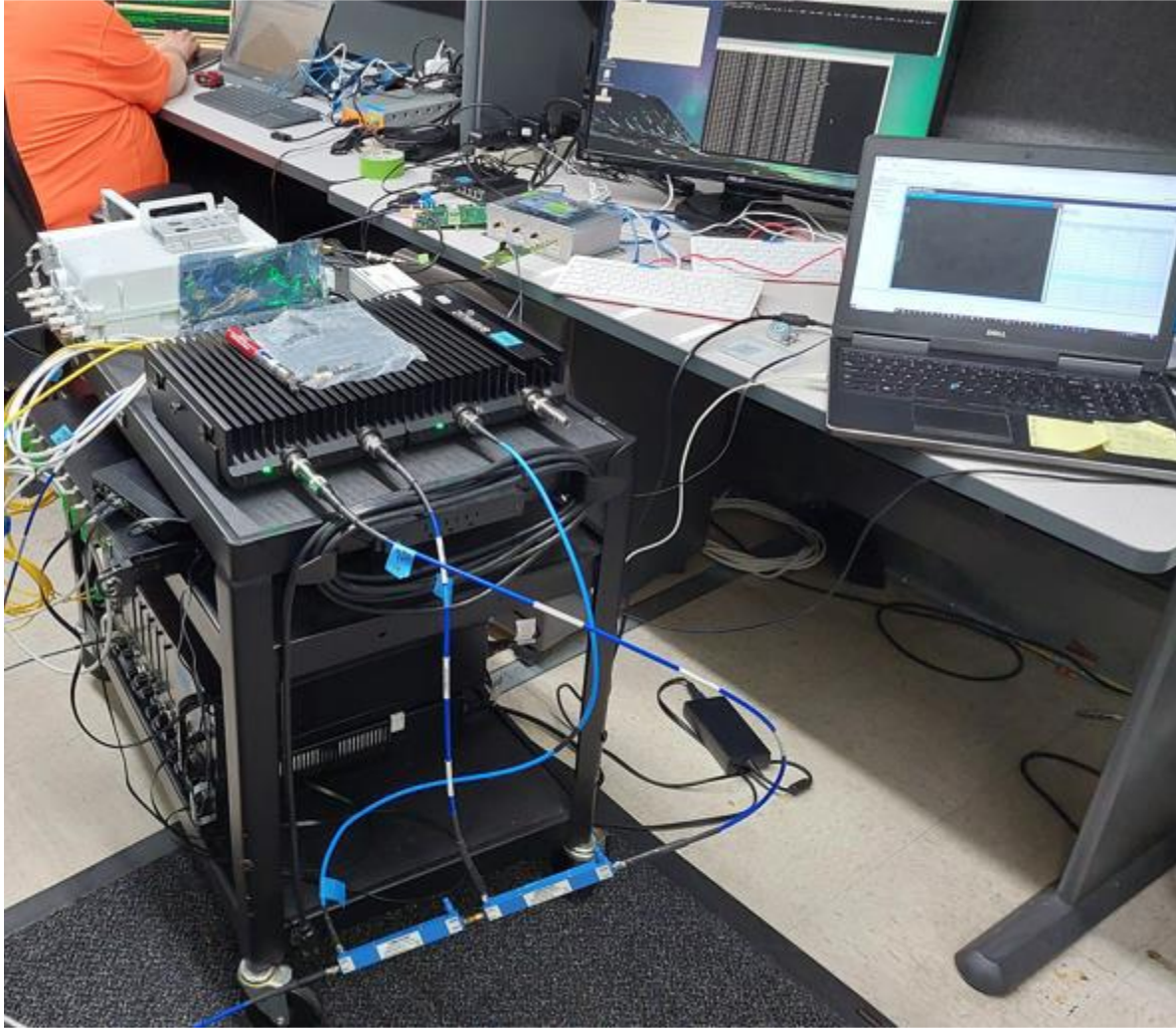
Figure 1 – CBSD-SAS Protocol Test Setup
