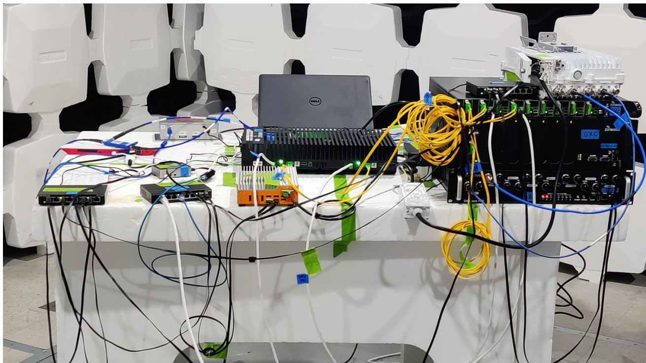
Figure 2 – Band 48 Radiated Spurious Emission Test Set Up: 30MHz – 1GHz
