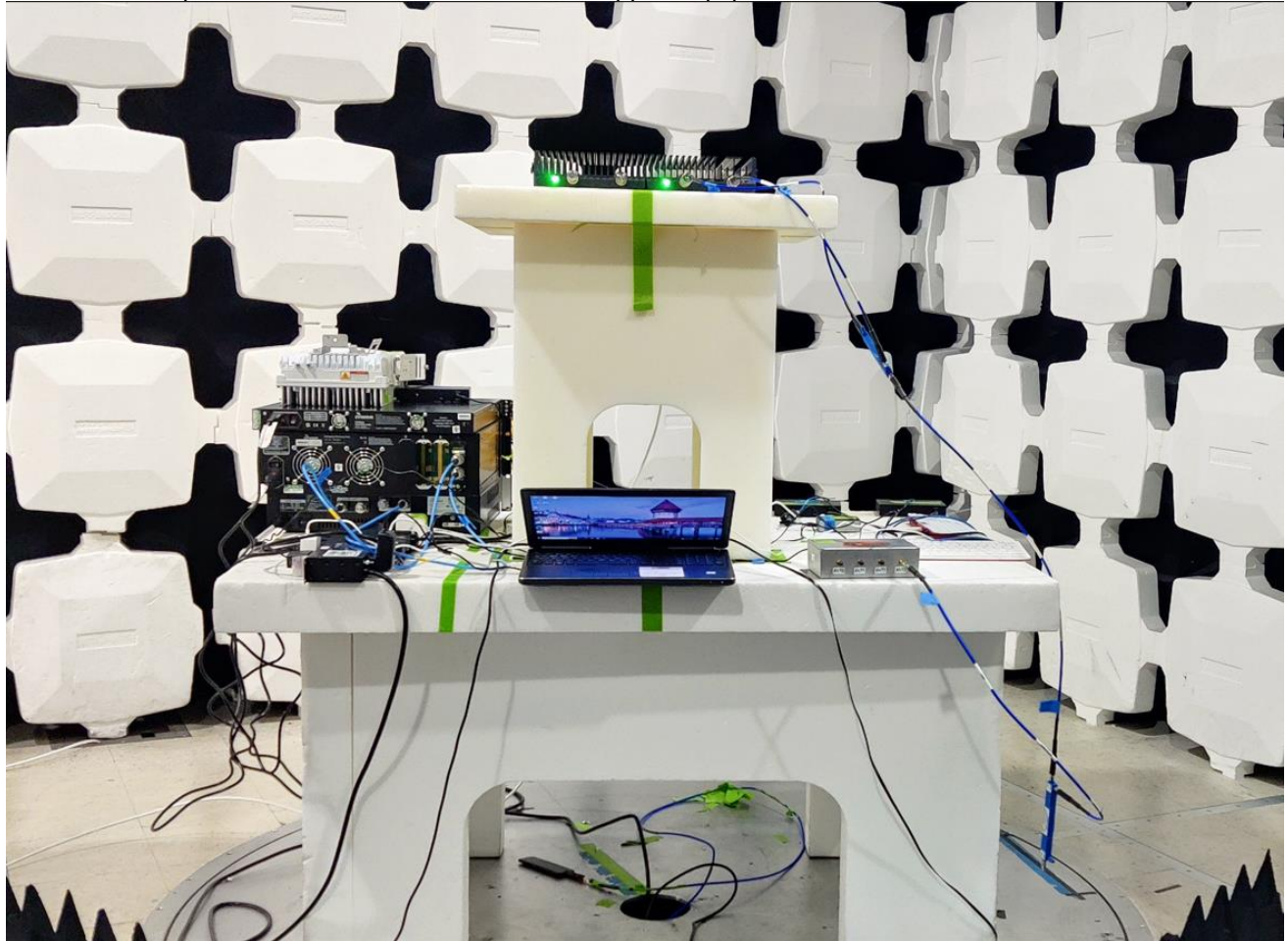
Figure 1 – Band 48 Radiated Spurious Emission Test Set Up: 1-18 GHz
