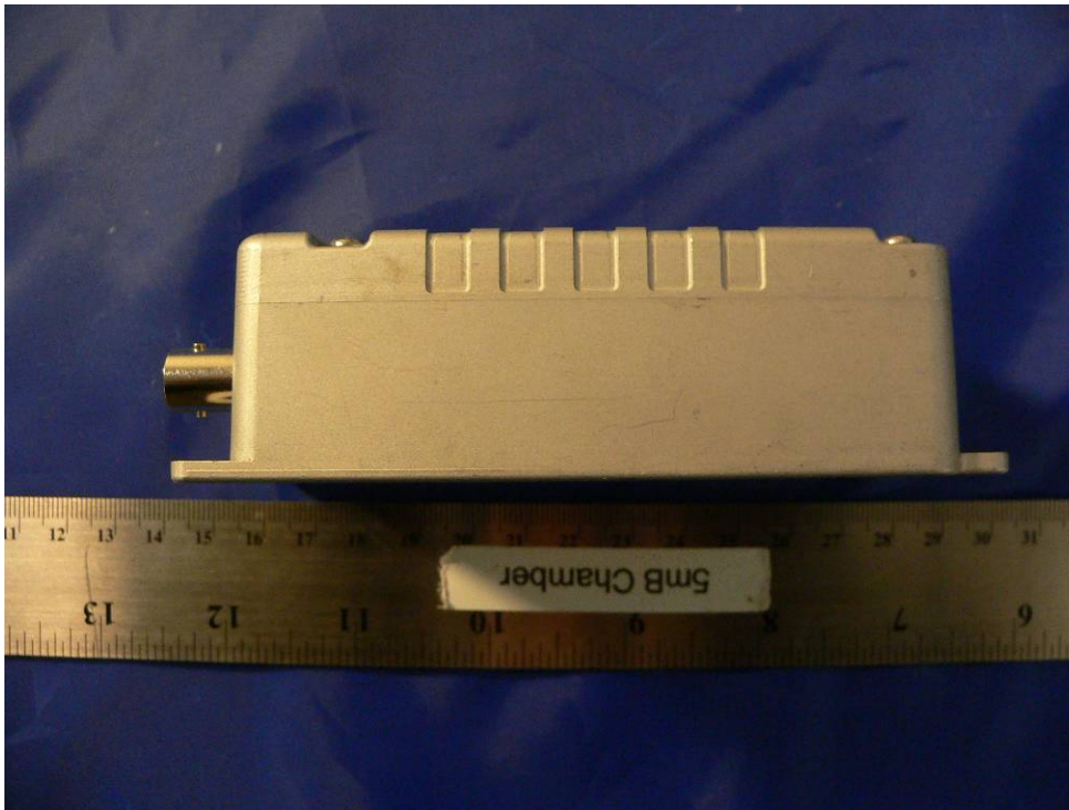
UHF: EUT-Port View
