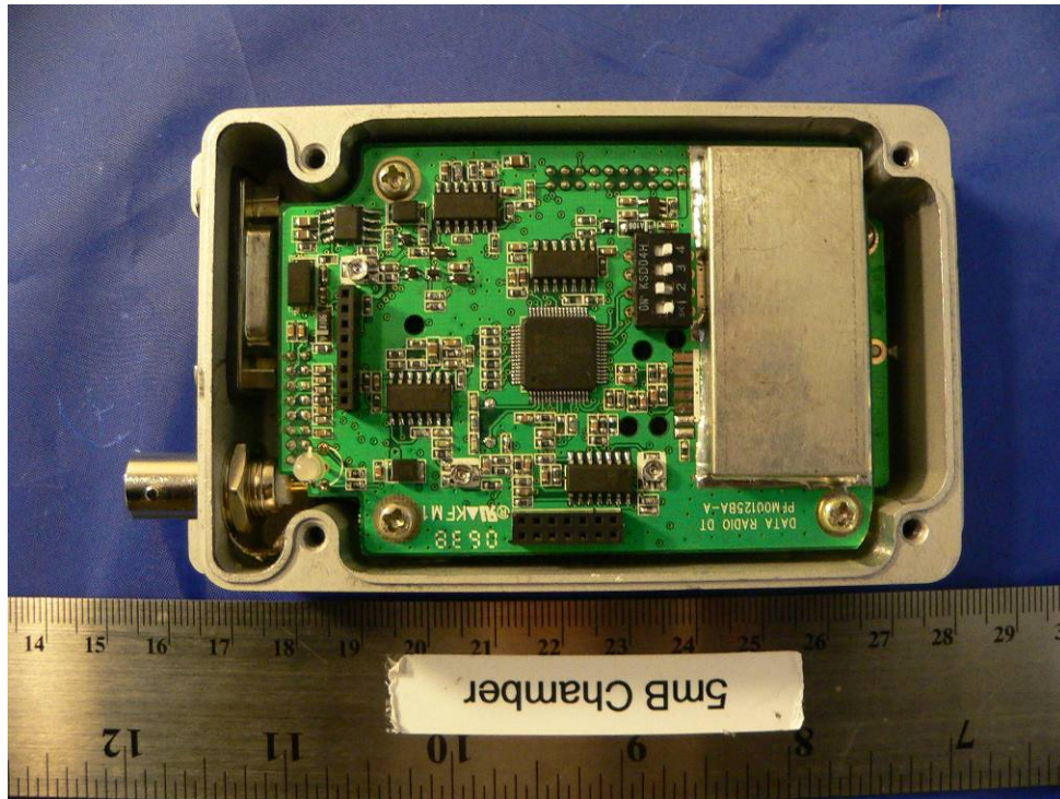
PCB1 Cover off Front view
