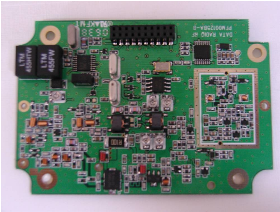
PCB2 - Without Shield – Front view
