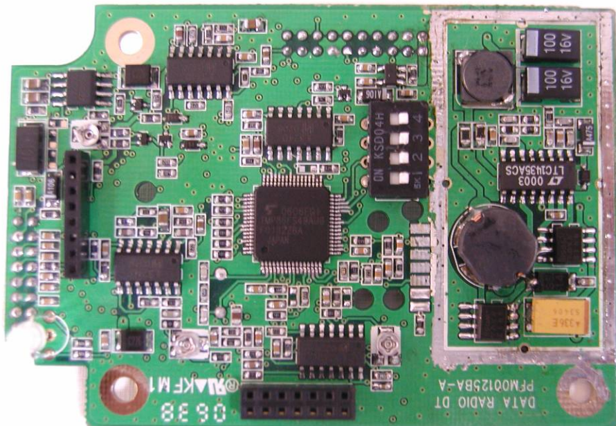
PCB1 without shield – Front view
