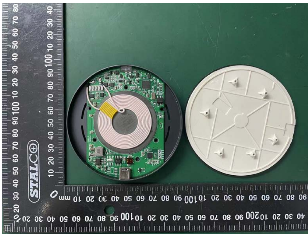
Internal photos M/N: WC15WGGLBLK-A
