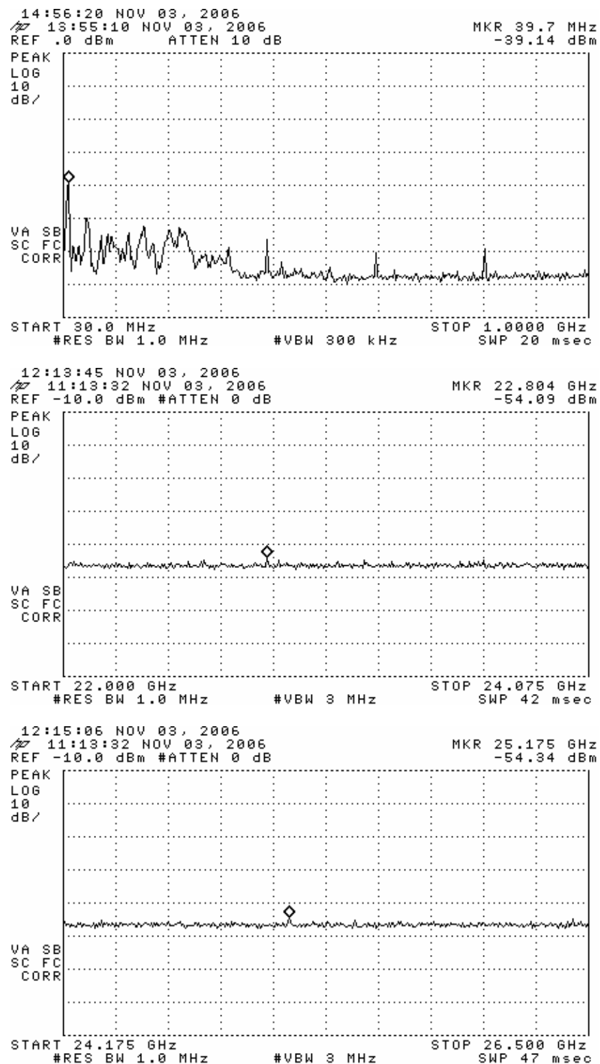
Figure 6.3. Digital/Spurious Emissions. (top) 30-1000 MHz, (middle) 22-24.075 GHz - noise, (bottom) 24.175-26.5 GHz - noise
