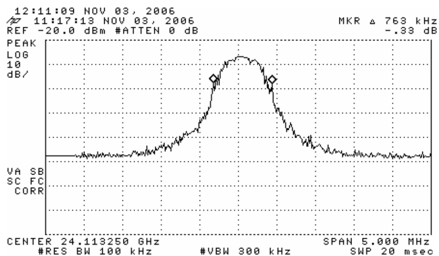
Figure 6.2. Fundamental Bandwidth Measurement.
