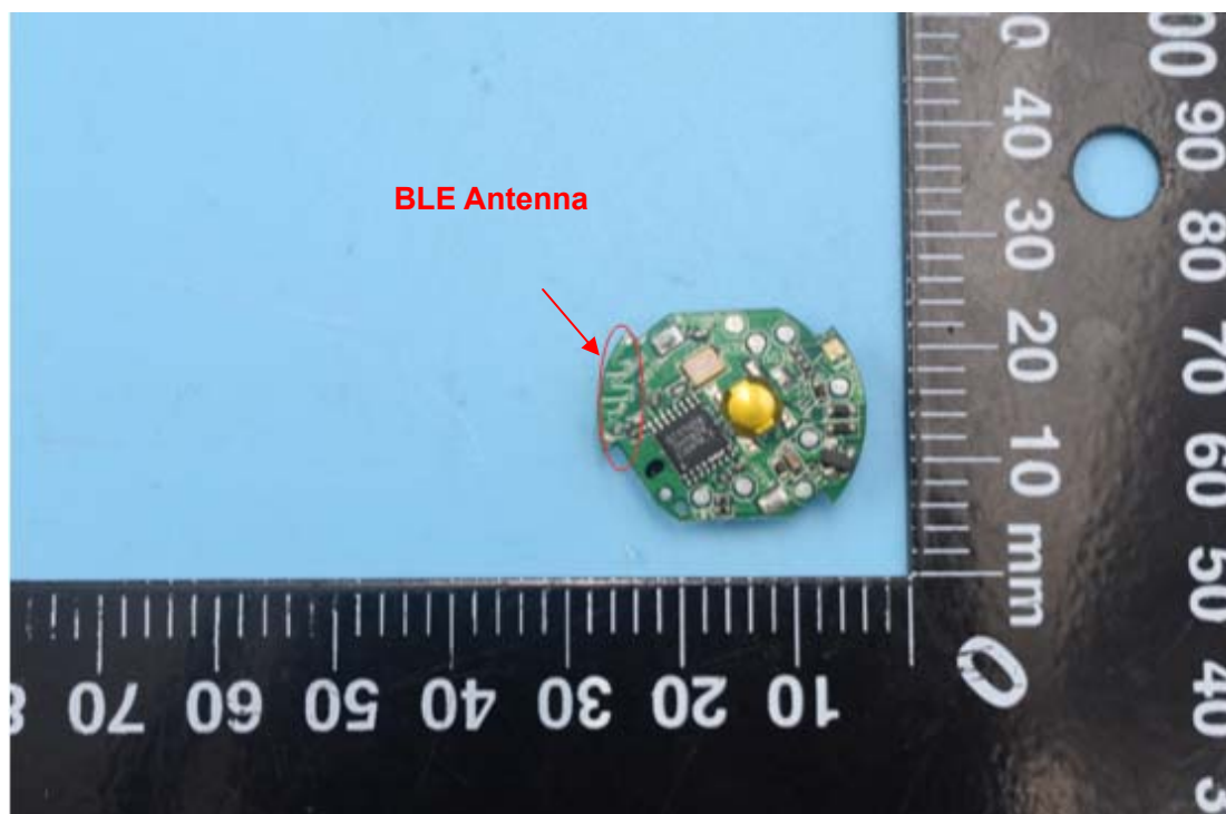
2. Antenna view
