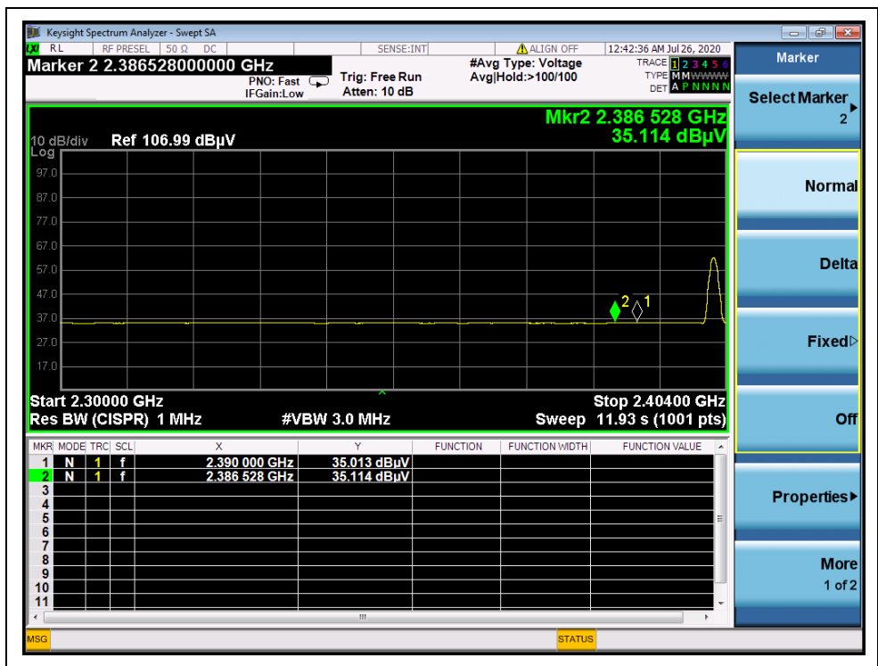
(AVG, Channel 0)
