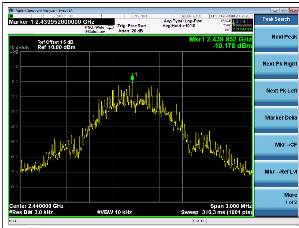
(Channel 19, 2440MHz)
