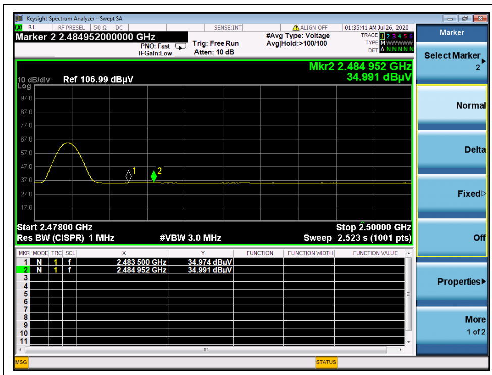
(AVG, Channel 39)
