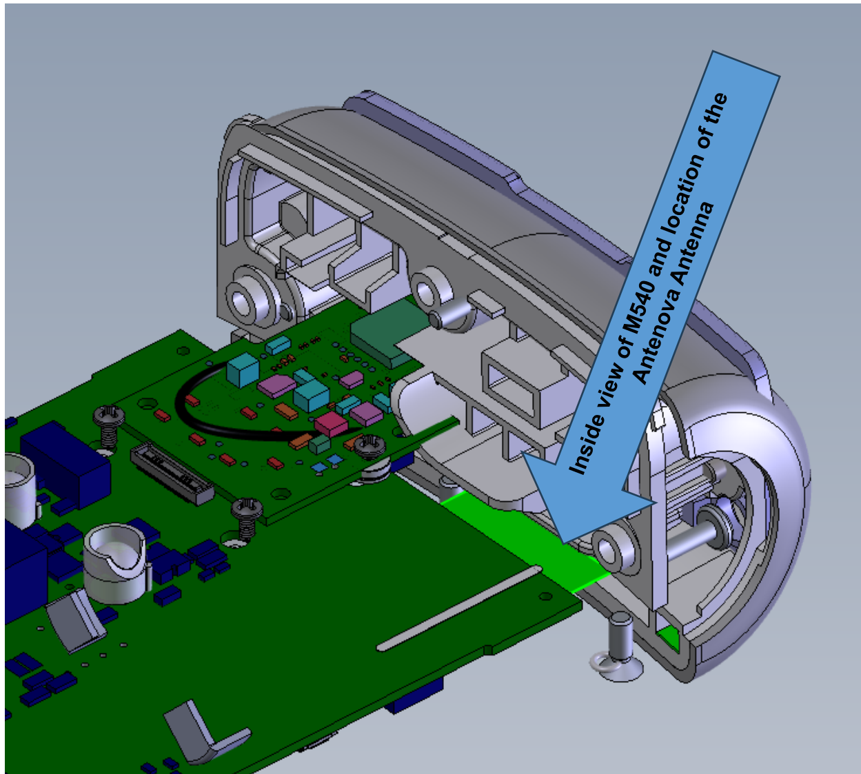
Figure 3 Inside view of M540 with Antenova Antenna in the end Cap.
