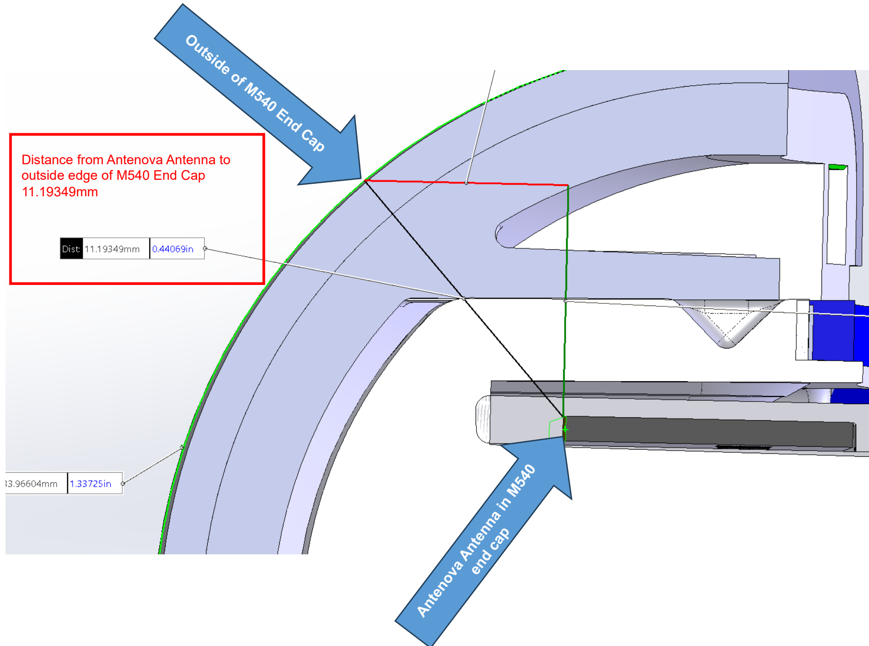
Figure 5 Measured shortest distance between Antanova antenna and outside case of M540 End Cap
