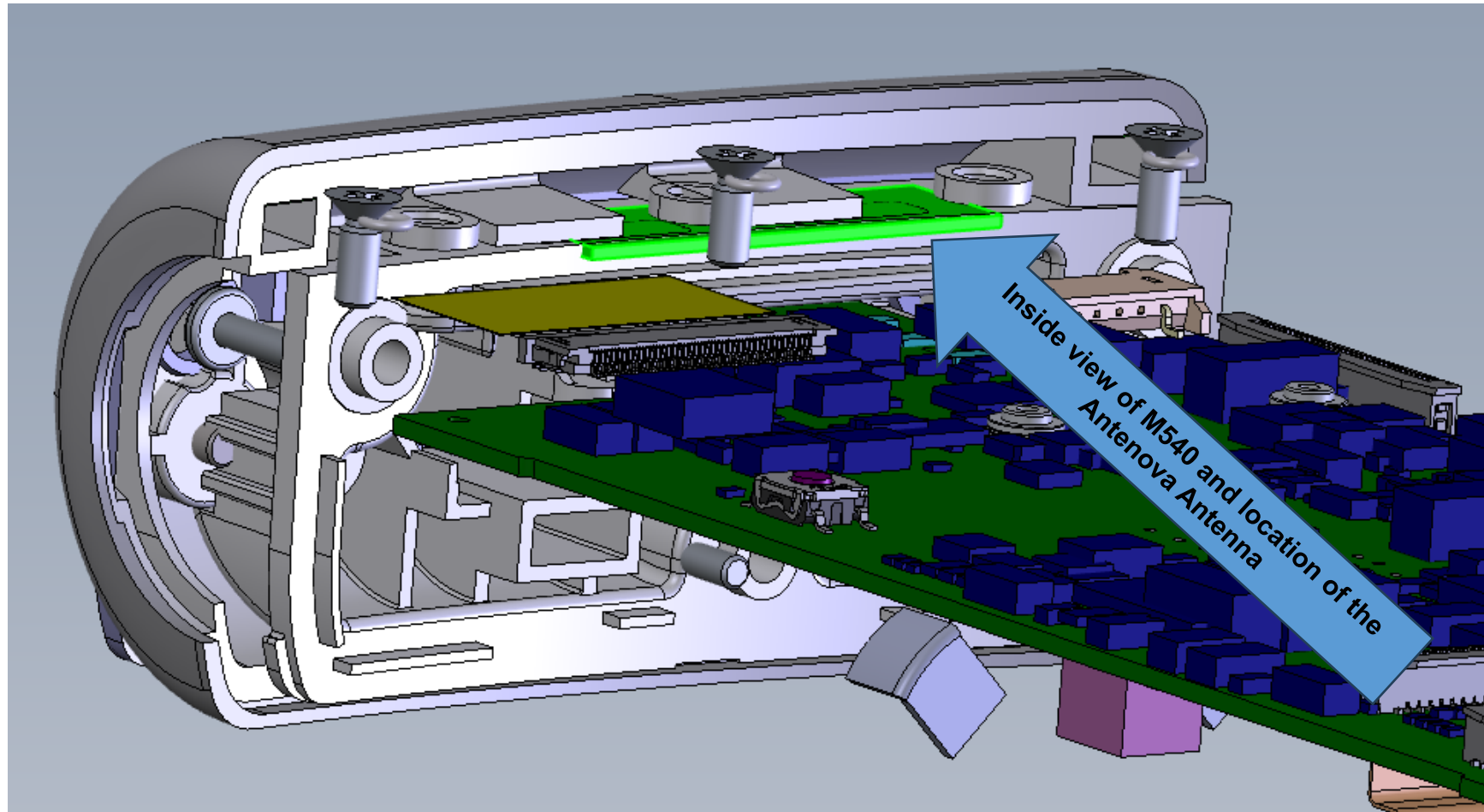
Figure 4 Inside view of M540 with Antenova Antenna in the End Cap
