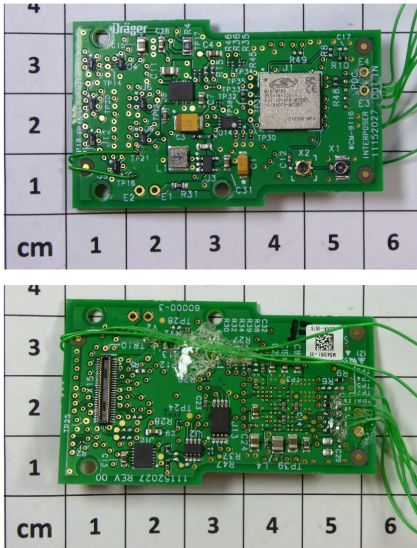
WCM 9116 with attached wires to access test modes:
