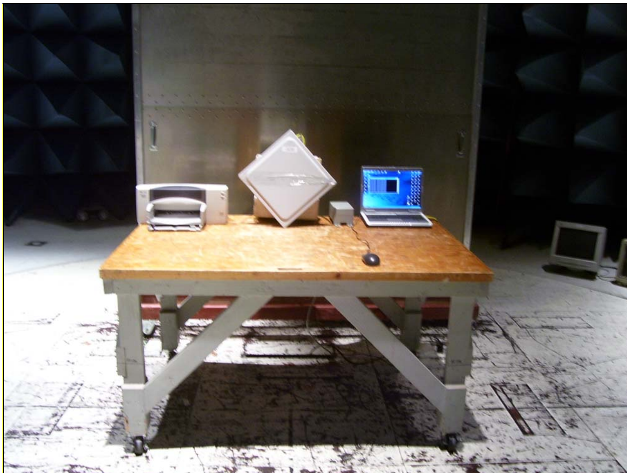
Photograph 3. Conducted Emissions Test Setup for ASN-700FCC-N
