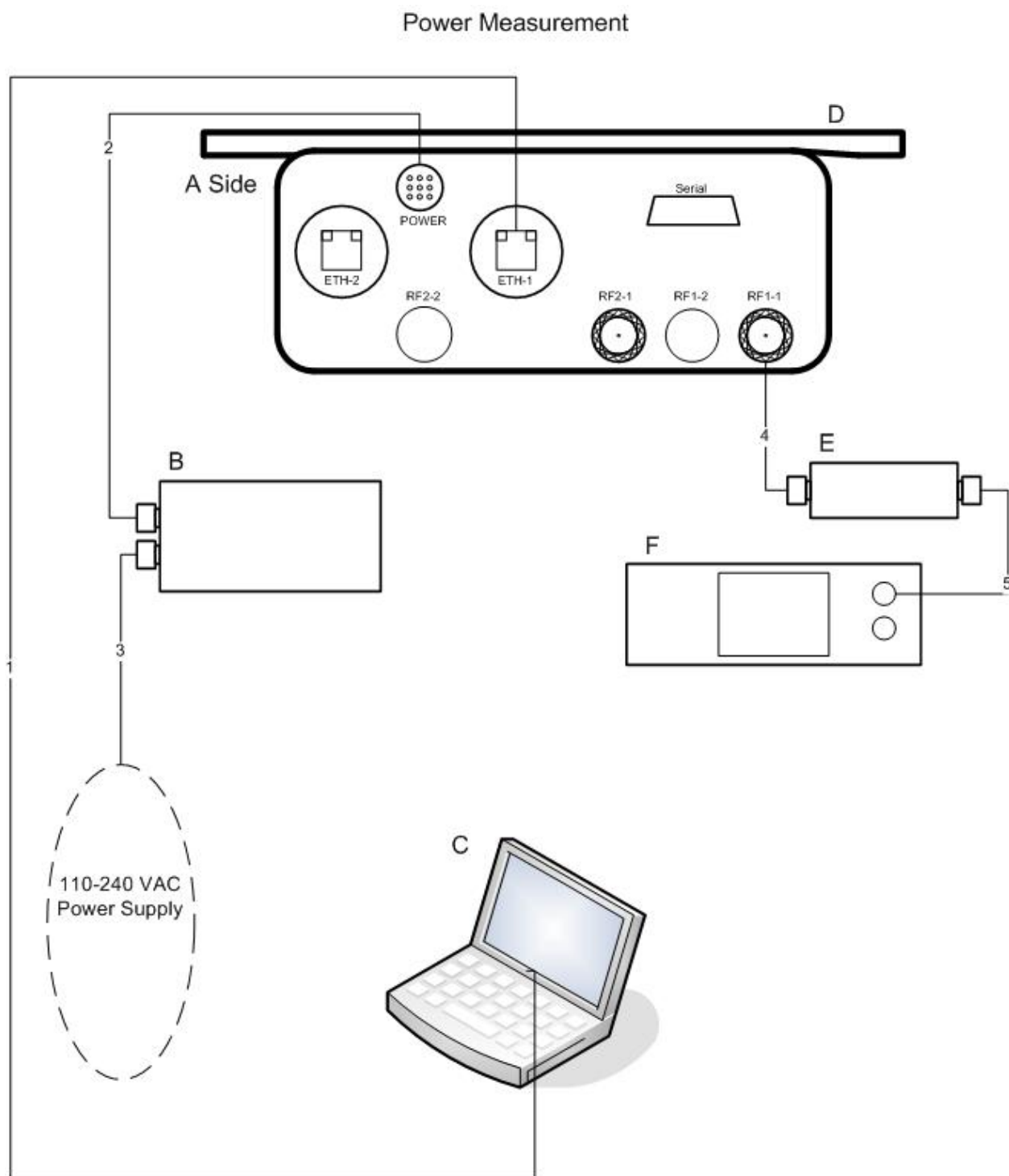
Figure 2. Block Diagram of Test Configuration – Conducted, Integral Antenna
