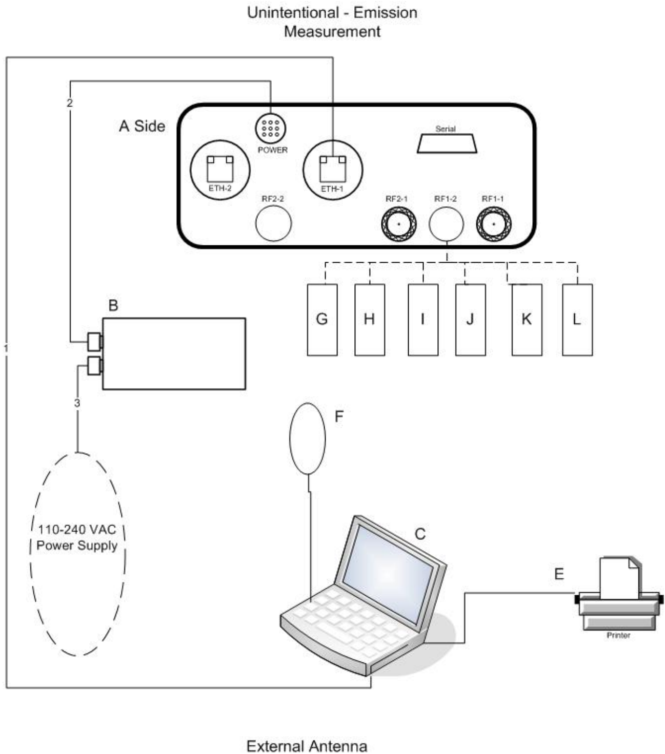
Figure 4. Block Diagram of Test Configuration – Unintentional Emissions, External Antenna
