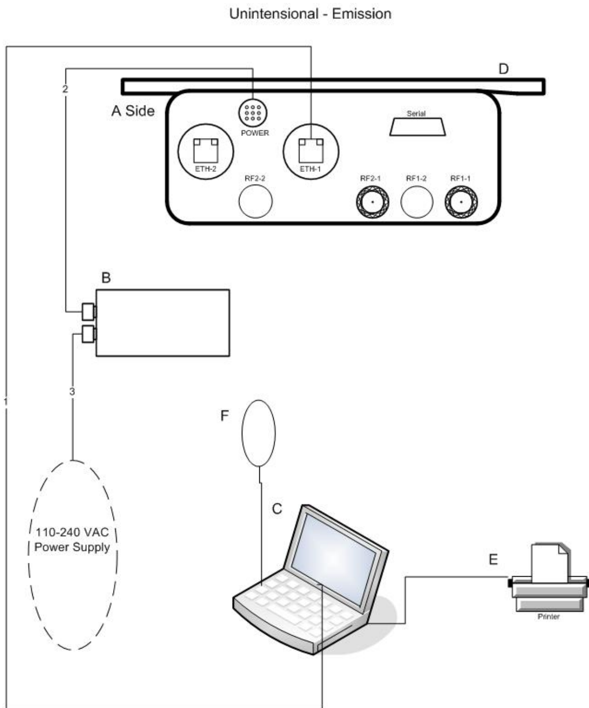
Figure 1. Block Diagram of Test Configuration – Unintentional Emissions, Integral Antenna
