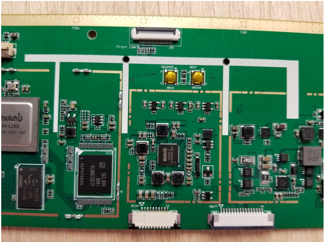
Photograph 17b - 2400-00429 main CPU assembly top side (Middle)
