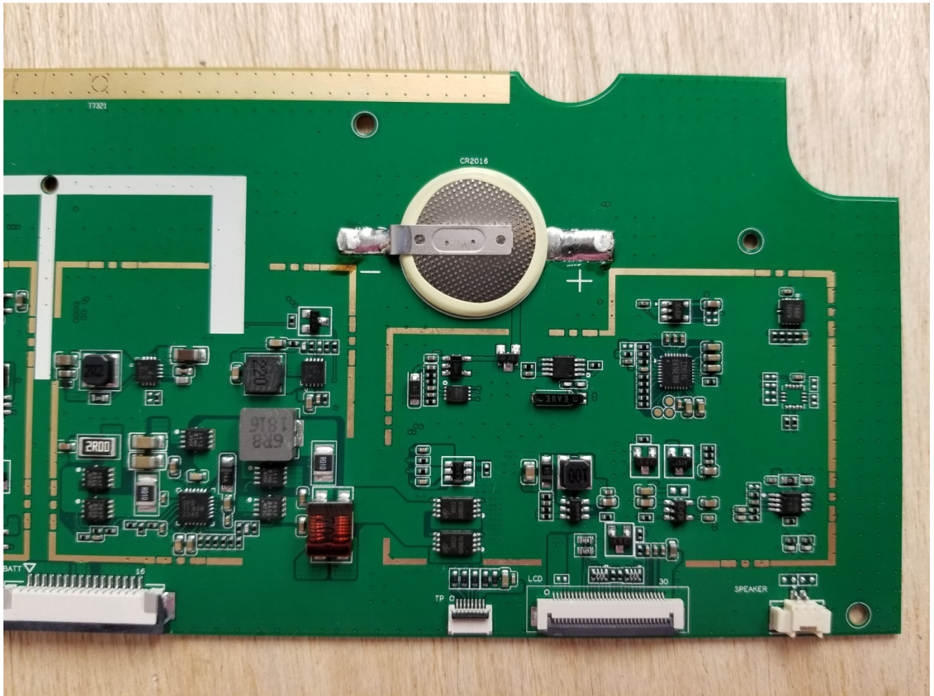
Photograph 18c - 2400-00429 main CPU assembly top side (Right Edge)
