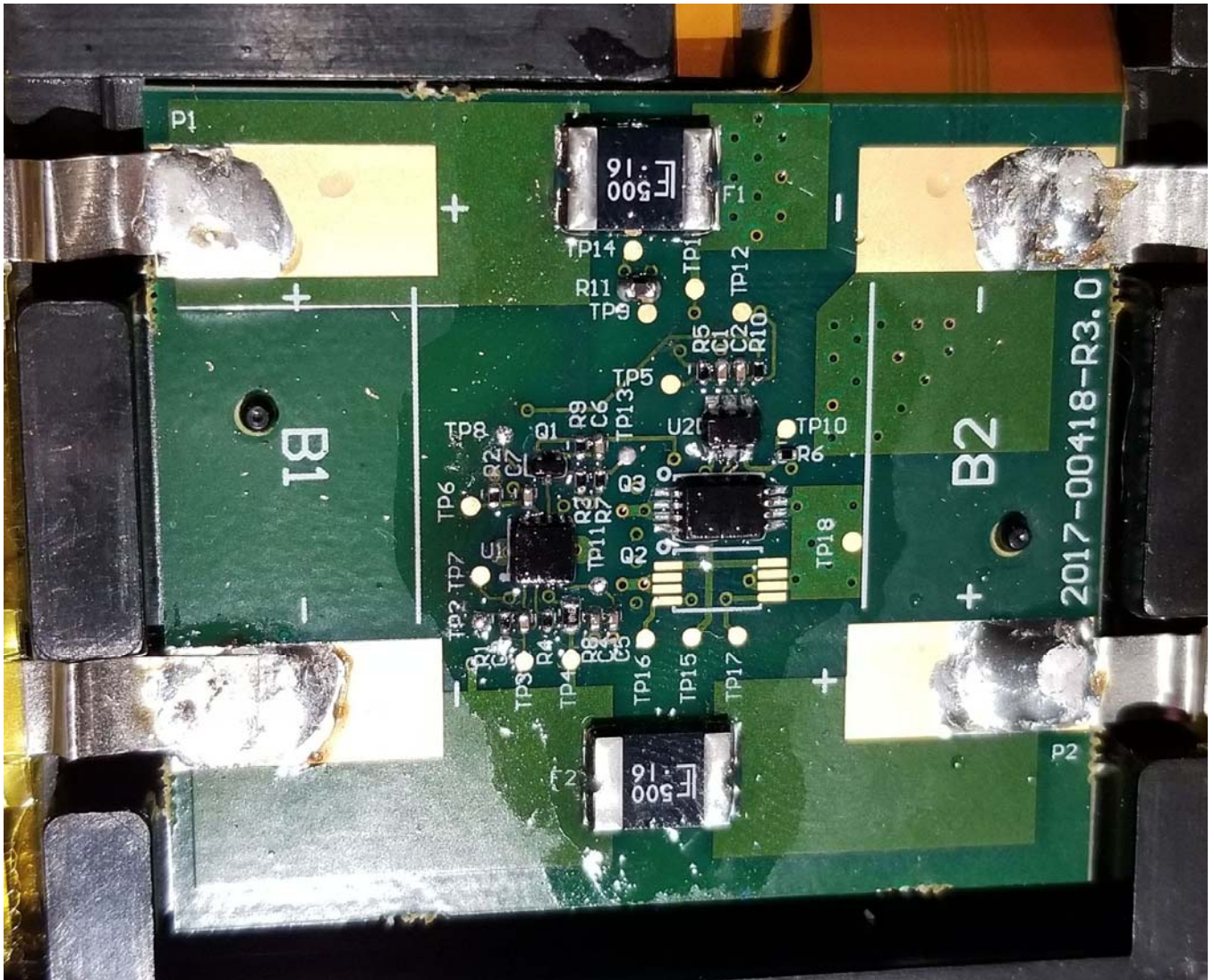
Photograph 28 – 2400-00428 Circuit detail
