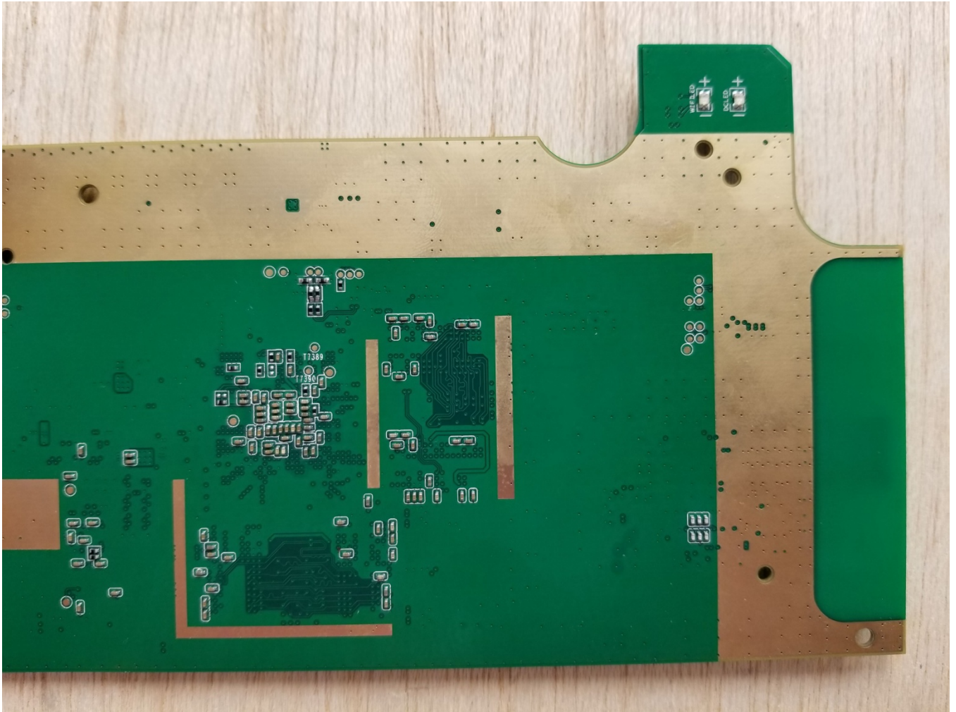
Photograph 19a - 2400-00429 main CPU bottom side (Left Edge)
