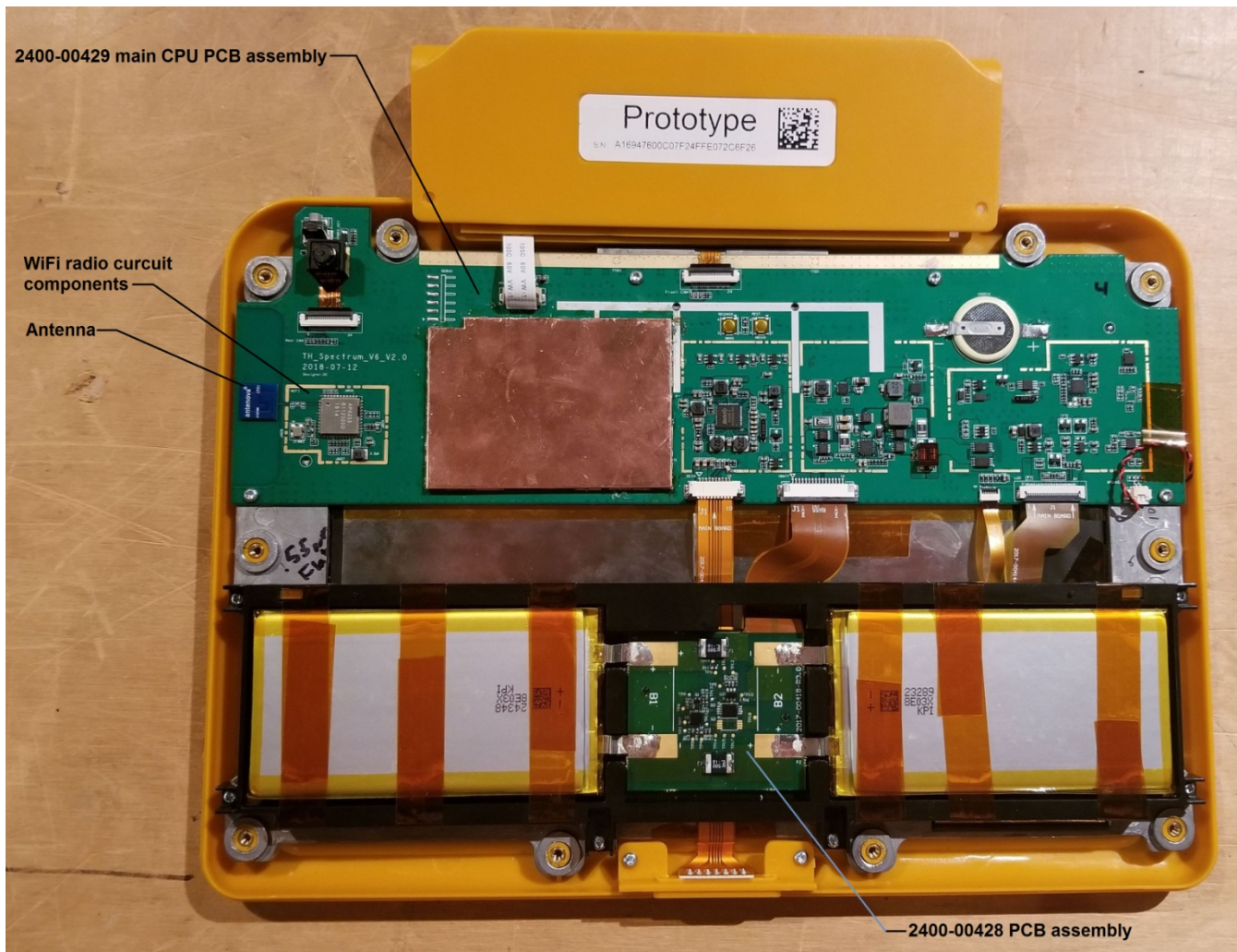
Photograph 29 - Pad6 Model: PHRPAD60 with back removed showing location of sub assemblies
