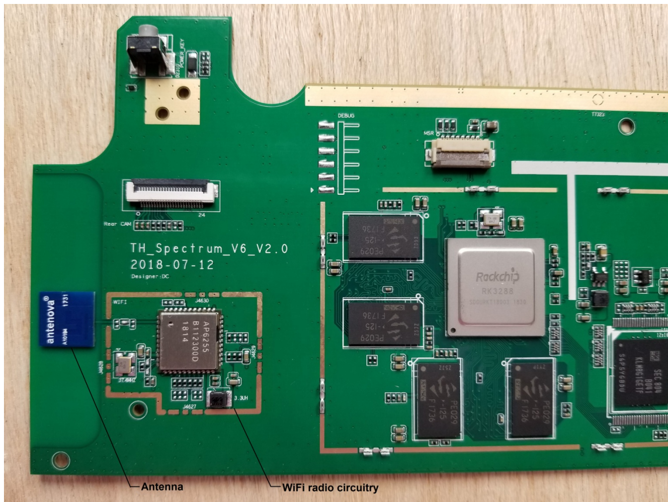
Photograph 16a – 2400-00429 main CPU assembly top side (Left Edge)
