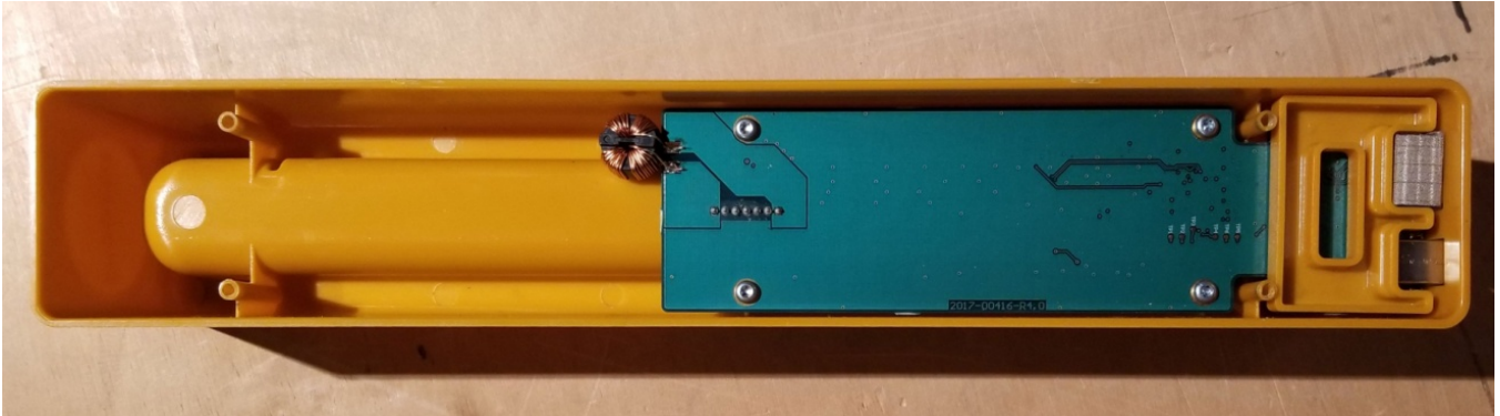
Photograph 22 - Ethernet docking cradle bottom view with bottom removed
