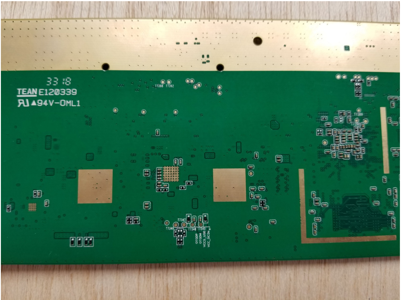
Photograph 20b - 2400-00429 main CPU bottom side (Middle)
