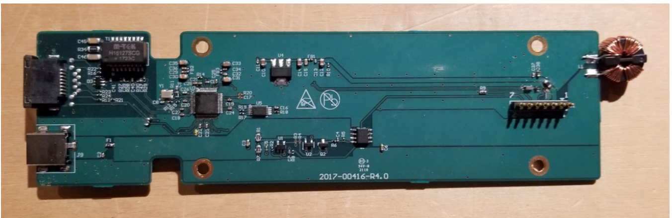
Photograph 23 - 2400-00427-R6 Ethernet docking cradle circuit board top side
