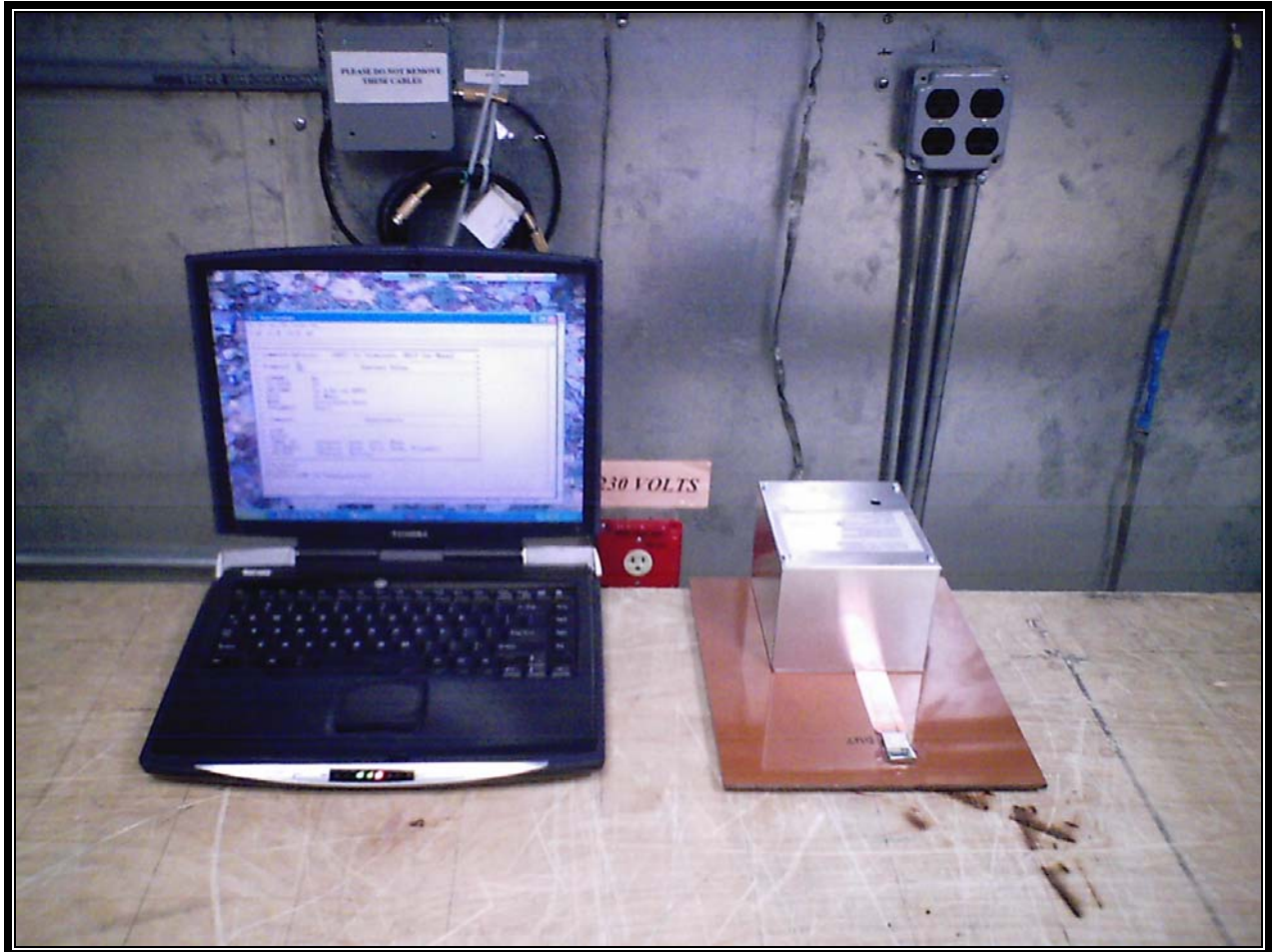
Photograph 3: AC Conducted Emissions Testing – Front View
