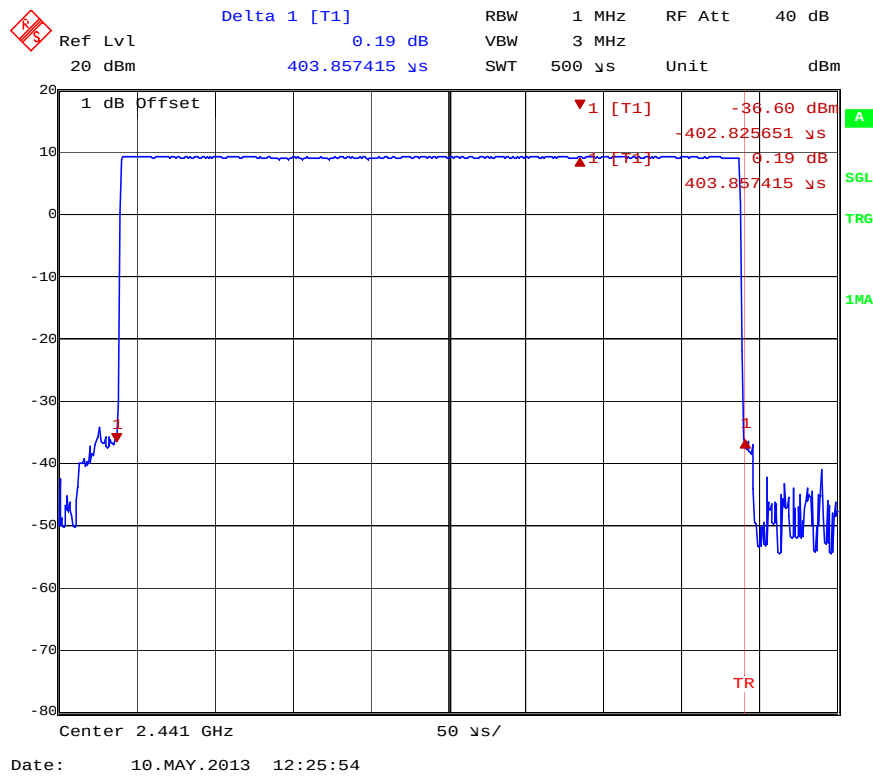
Channel Occupancy Time (1Mbps)
