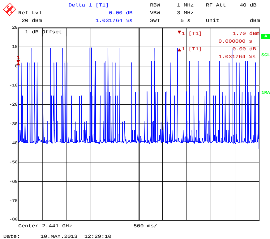
Number of Transmissions in 5 Seconds (1Mbps)
