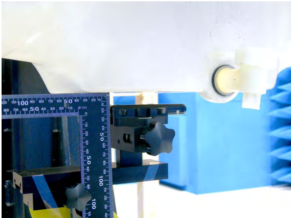
Figure 17. Body SAR Test Setup (Flat Section)
