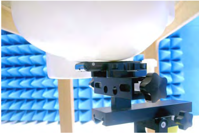
Figure 13. Right Head SAR Test Setup (Cheek)
