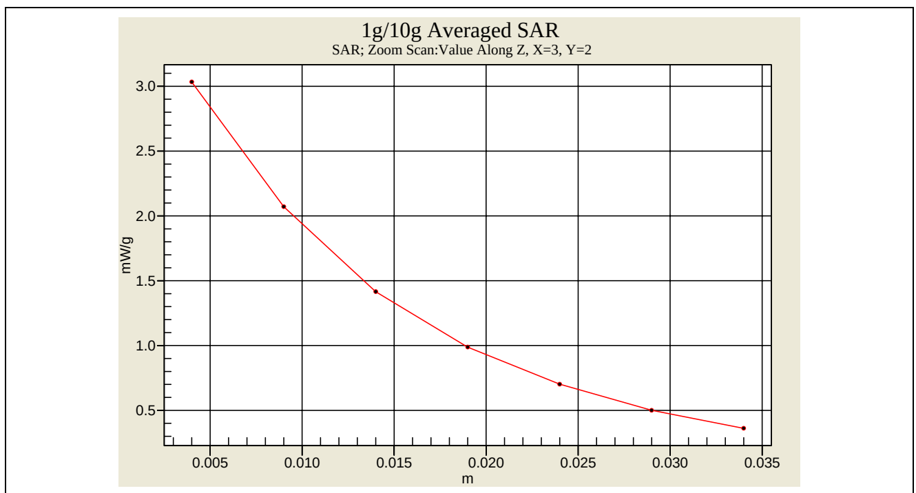
Body-Tissue-Simulating-Liquid 900MHz
