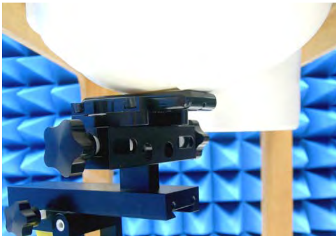
Figure 15. Left Head SAR Test Setup (Cheek)
