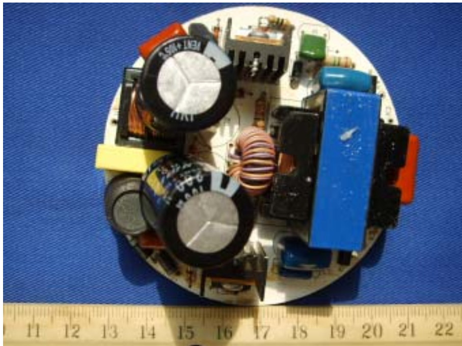
EUT –Components View
