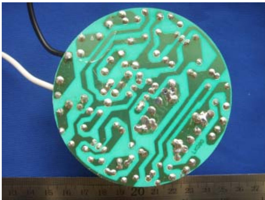
EUT–Solder View
