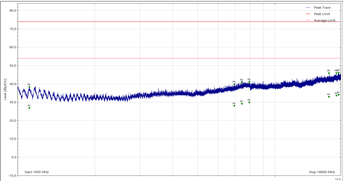
Figure 6 - 1 GHz to 18 GHz, Peak & CISPR Average, Horizontal
