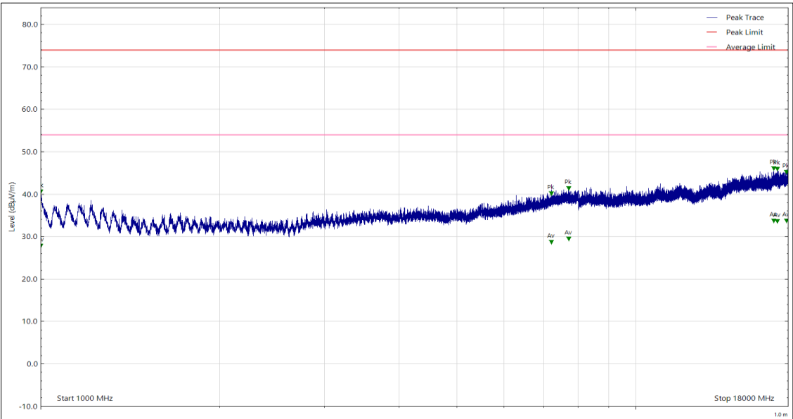
Figure 7 - 1 GHz to 18 GHz, Peak & CISPR Average, Vertical
