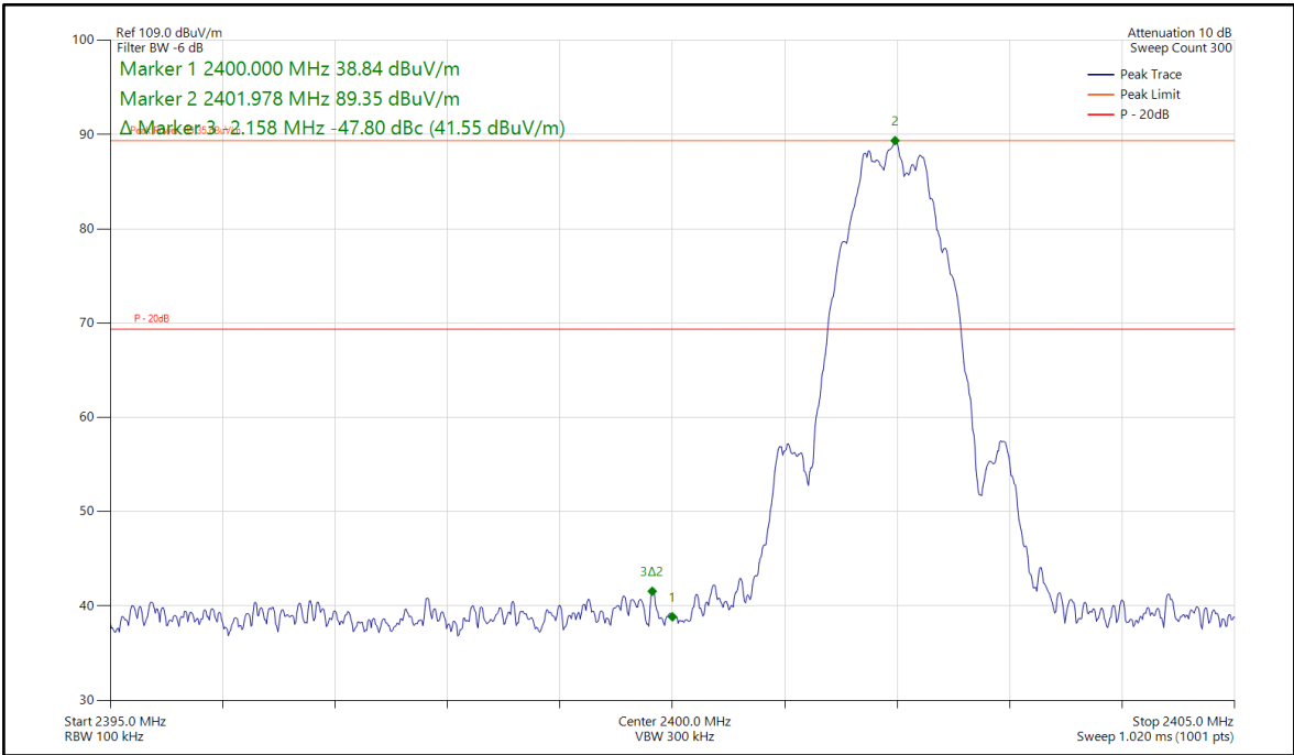
Figure 7 - BLE, 2402 MHz, Band Edge Frequency 2400 MHz
