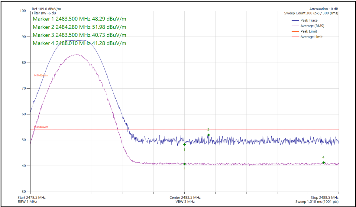
Figure 2 - BLE, 2480 MHz, Band Edge Frequency 2483.5 MHz
