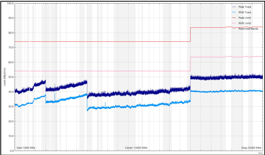
Figure 17 - CH19_LE1M, 2440 MHz, 1 GHz to 25 GHz, Vertical
