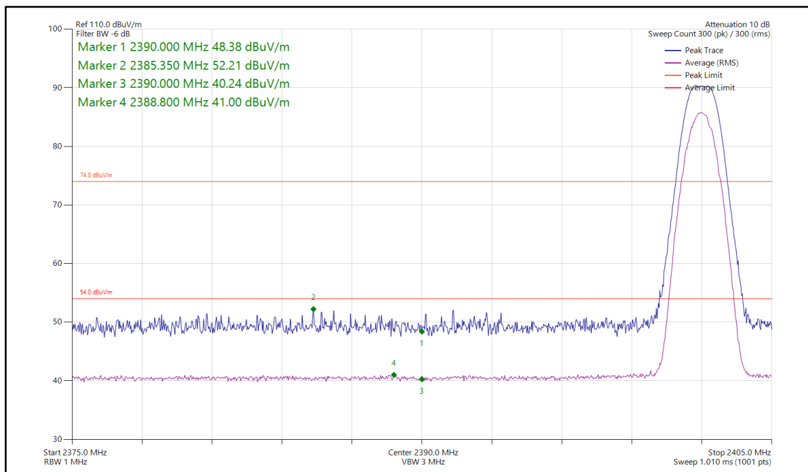
Figure 1 - BLE, 2402 MHz, Band Edge Frequency 2390 MHz
