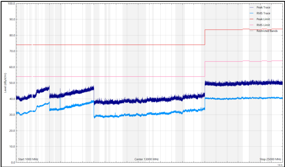
Figure 19 - CH39_LE1M, 2480 MHz, 1 GHz to 25 GHz, Horizontal
