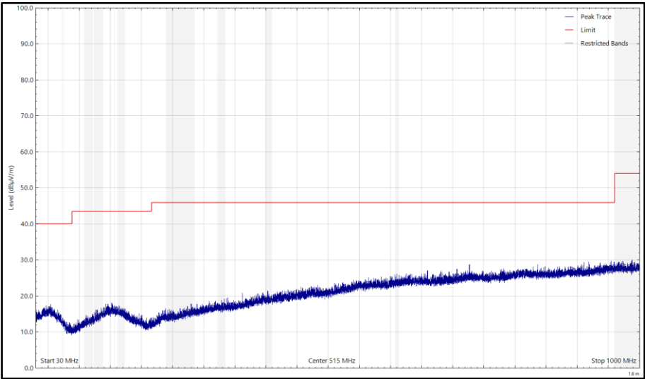
Figure 12 - CH37_LE1M, 2402 MHz, 30 MHz to 1 GHz, Vertical (Peak)
