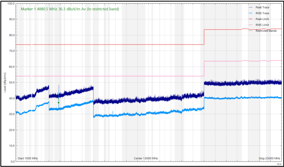
Figure 15 - CH19_LE1M, 2440 MHz, 1 GHz to 25 GHz, Horizontal
