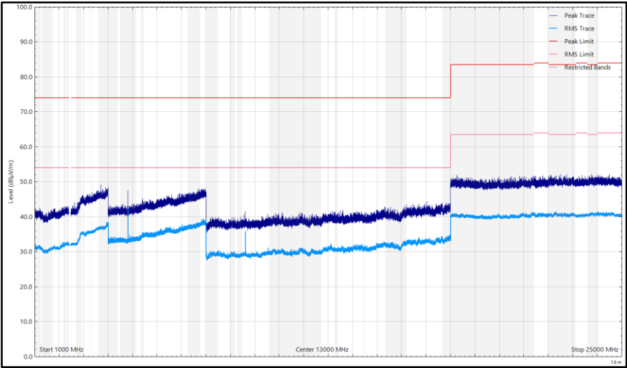
Figure 11 - CH37_LE1M, 2402 MHz, 1 GHz to 25 GHz, Horizontal
