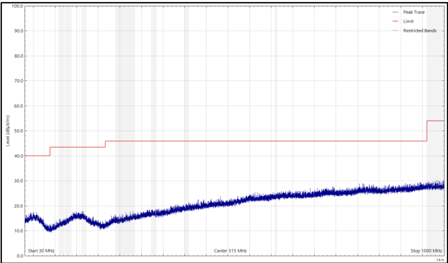
Figure 10 - CH37_LE1M, 2402 MHz, 30 MHz to 1 GHz, Horizontal (Peak)
