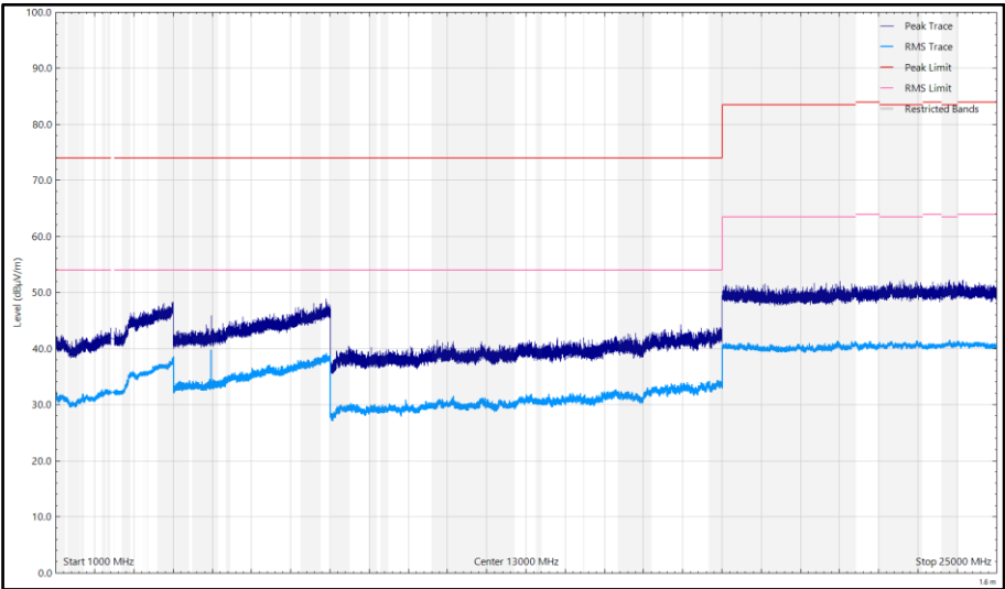
Figure 21 - CH39_LE1M, 2480 MHz, 1 GHz to 25 GHz, Vertical
