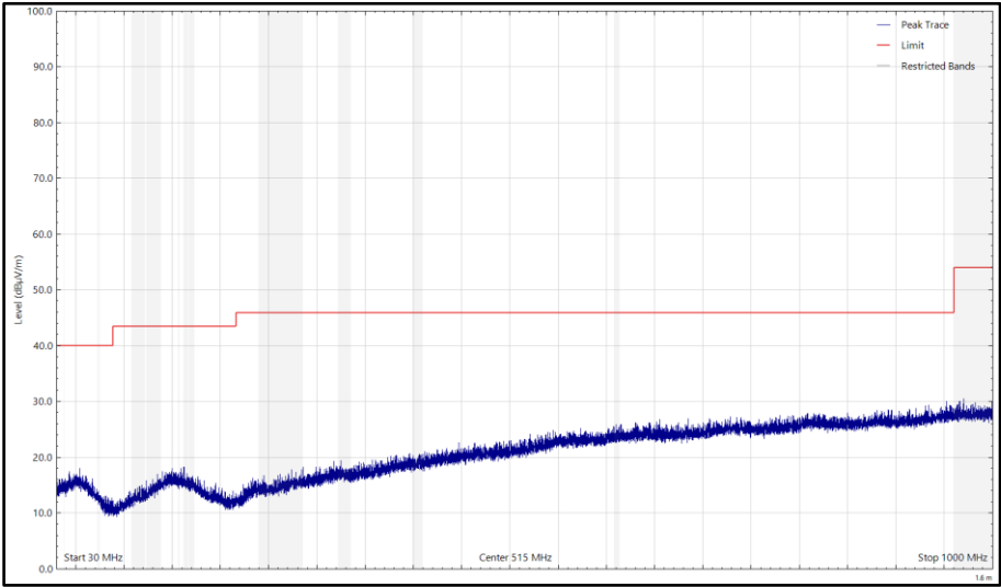
Figure 18 - CH39_LE1M, 2480 MHz, 30 MHz to 1 GHz, Horizontal (Peak)
