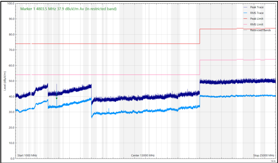
Figure 13 - CH37_LE1M, 2402 MHz, 1 GHz to 25 GHz, Vertical
