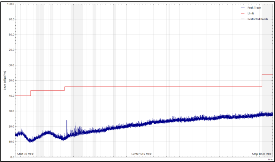
Figure 14 - CH19_LE1M, 2440 MHz, 30 MHz to 1 GHz, Horizontal (Peak)
