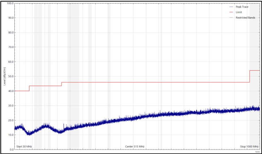
Figure 16 - CH19_LE1M, 2440 MHz, 30 MHz to 1 GHz, Vertical (Peak)
