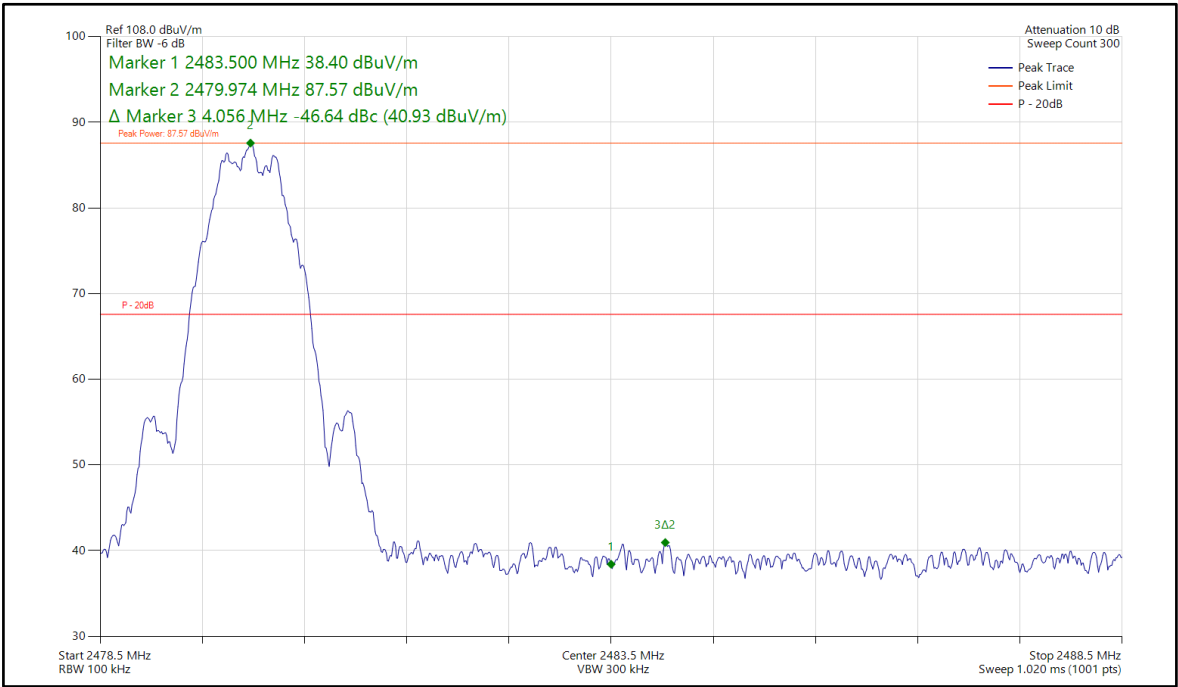
Figure 8 - BLE, 2480 MHz, Band Edge Frequency 2483.5 MHz
