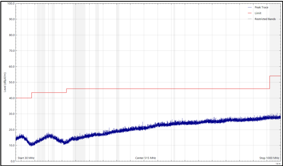
Figure 20 - CH39_LE1M, 2480 MHz, 30 MHz to 1 GHz, Vertical (Peak)
