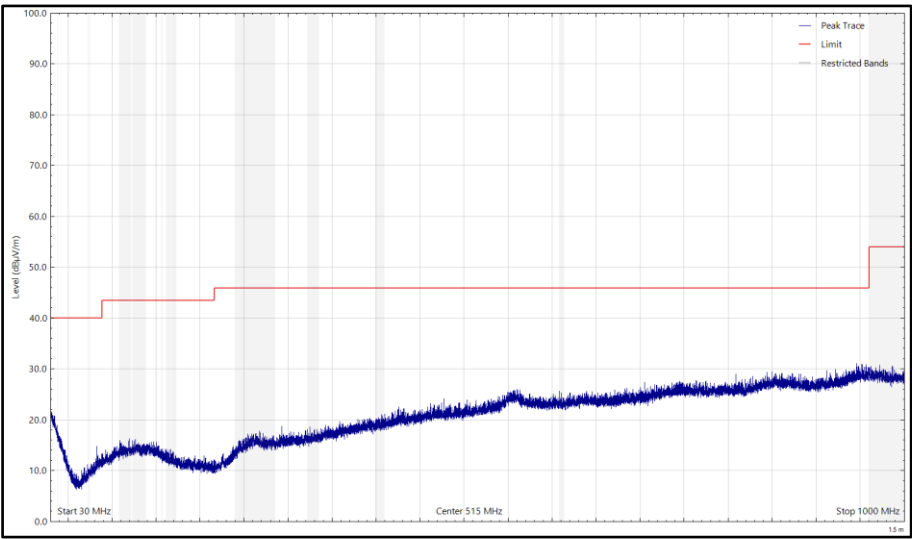
Figure 8 - SimTx_NFC_BLE, 13.56MHz_2438MHz, 30 MHz to 1 GHz, Vertical (Peak)
