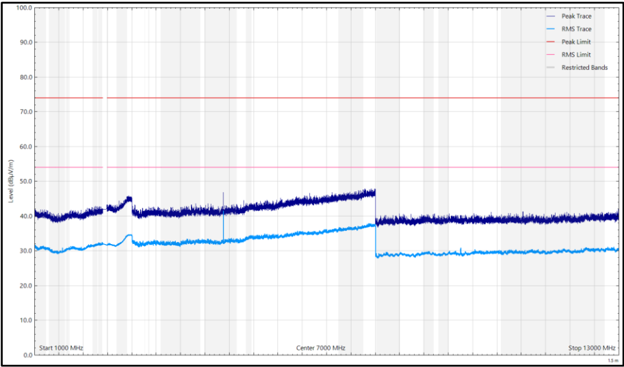
Figure 7 - SimTx_NFC_BLE, 13.56MHz_2438MHz, 1 GHz to 13 GHz, Horizontal
