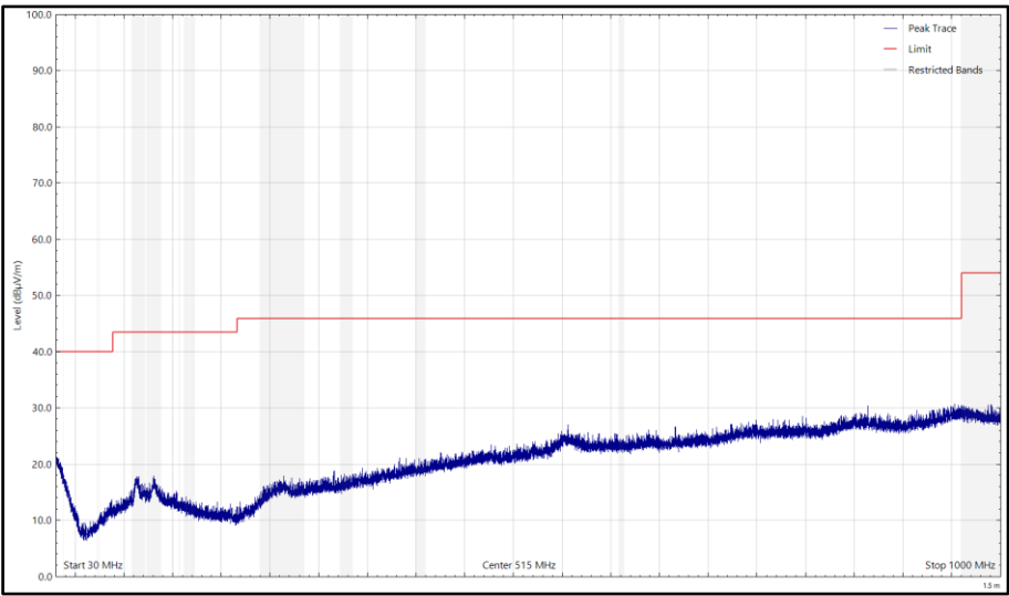
Figure 6 - SimTx_NFC_BLE, 13.56MHz_2438MHz, 30 MHz to 1 GHz, Horizontal (Peak)
