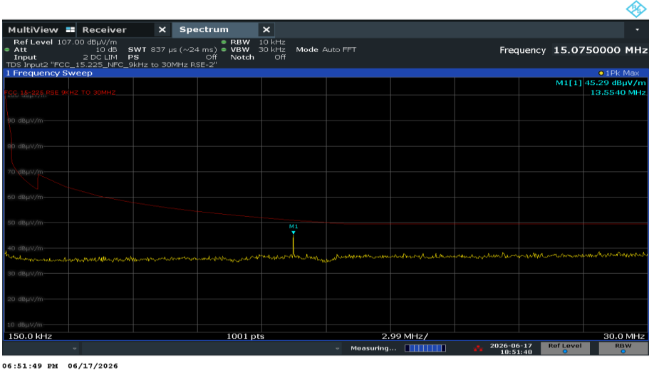
Figure 5 - SimTx_NFC_BLE, 13.56MHz_2438MHz, 150 kHz to 30 MHz, Side-On
