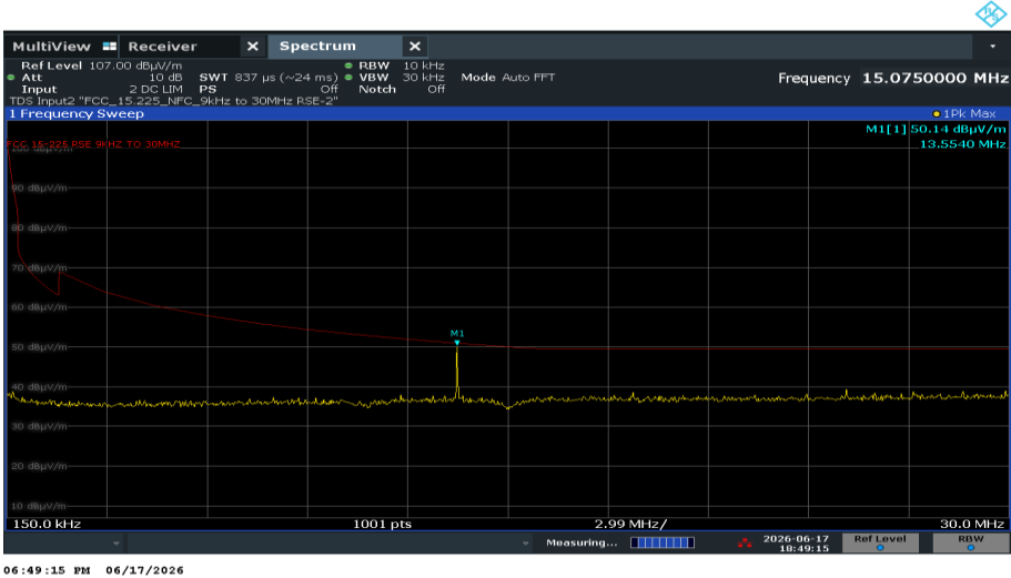
Figure 4 - SimTx_NFC_BLE, 13.56MHz_2438MHz, 150 kHz to 30 MHz, Front-On
