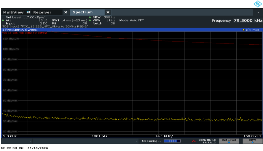
Figure 3 - SimTx_NFC_BLE, 13.56MHz_2438MHz, 9 kHz to 150 kHz, Side-On
