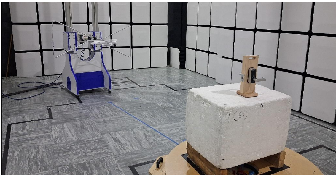
Figure 12 - Test Setup - 30 MHz to 1 GHz
