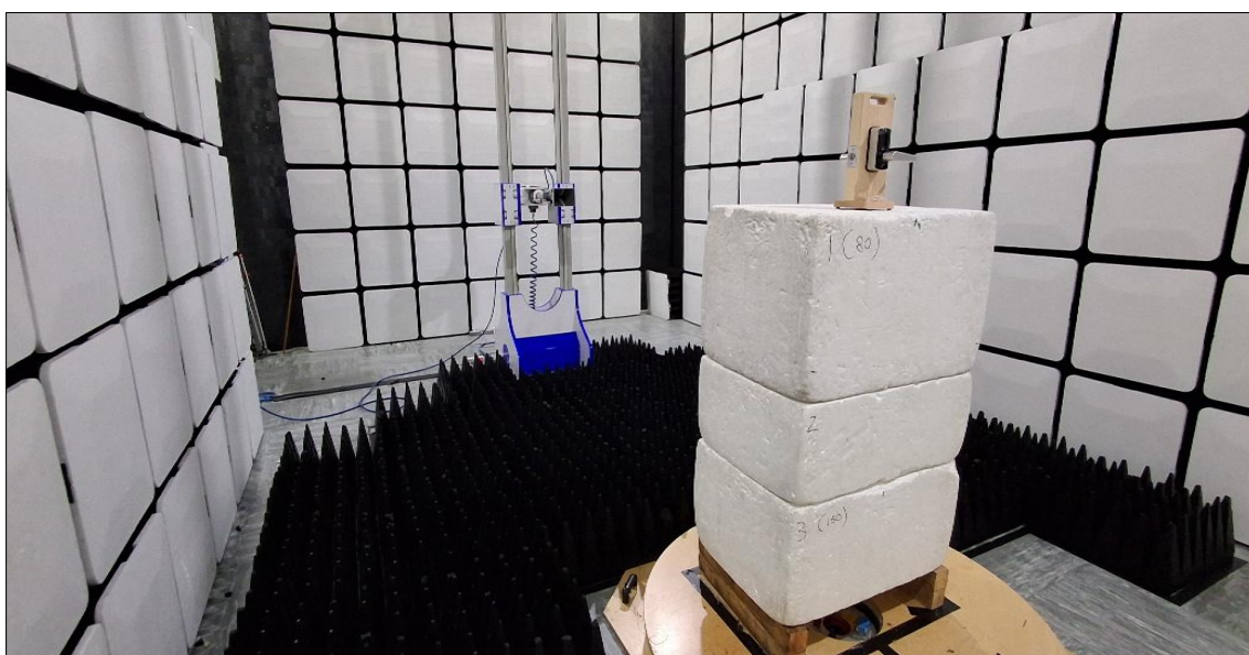
Figure 13 - Test Setup - 1 GHz to 8 GHz
