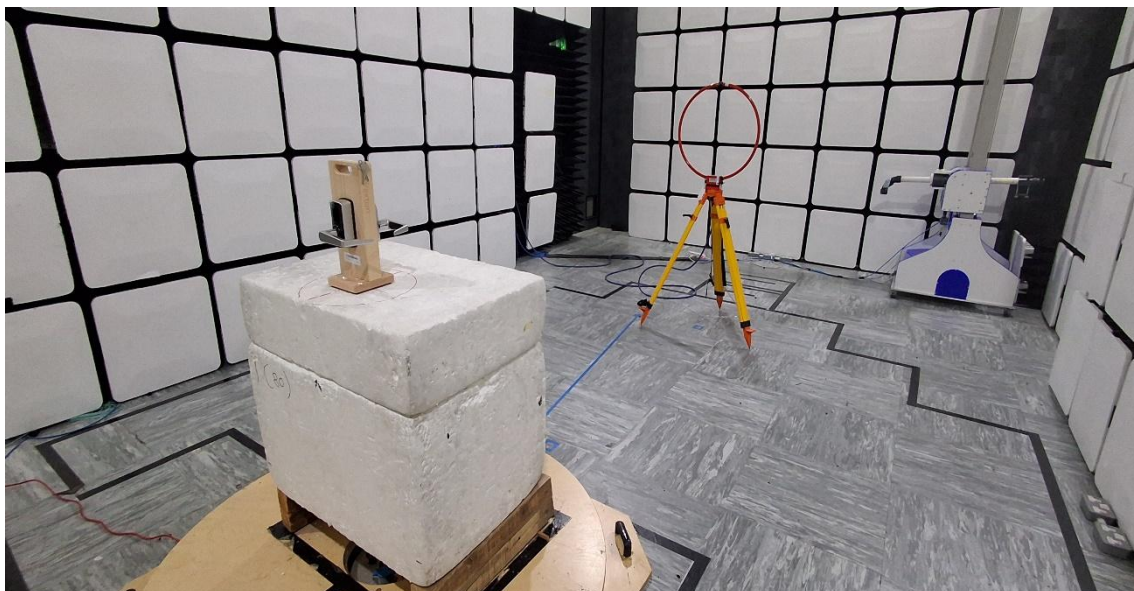
Figure 10 - Test Setup – 9kHz to 30MHz Front-On
