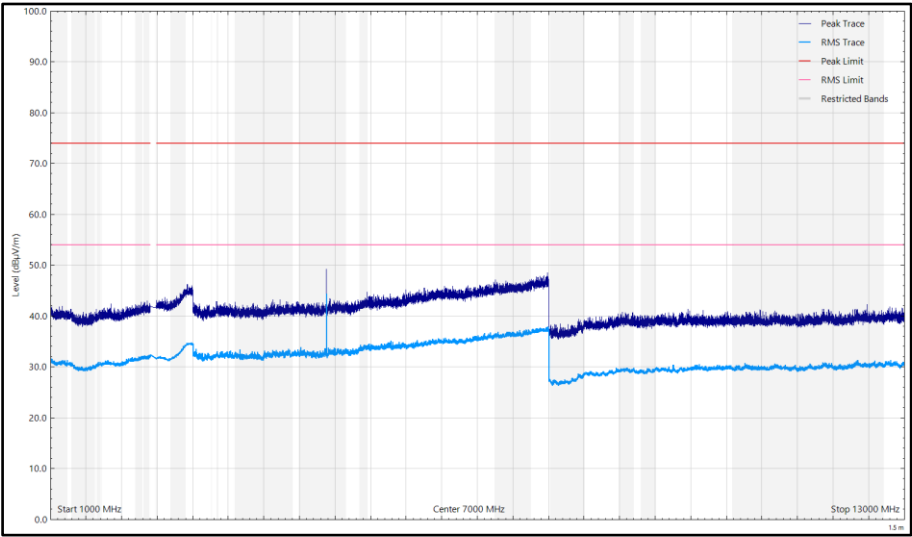
Figure 9 - SimTx_NFC_BLE, 13.56MHz_2438MHz, 1 GHz to 13 GHz, Vertical
