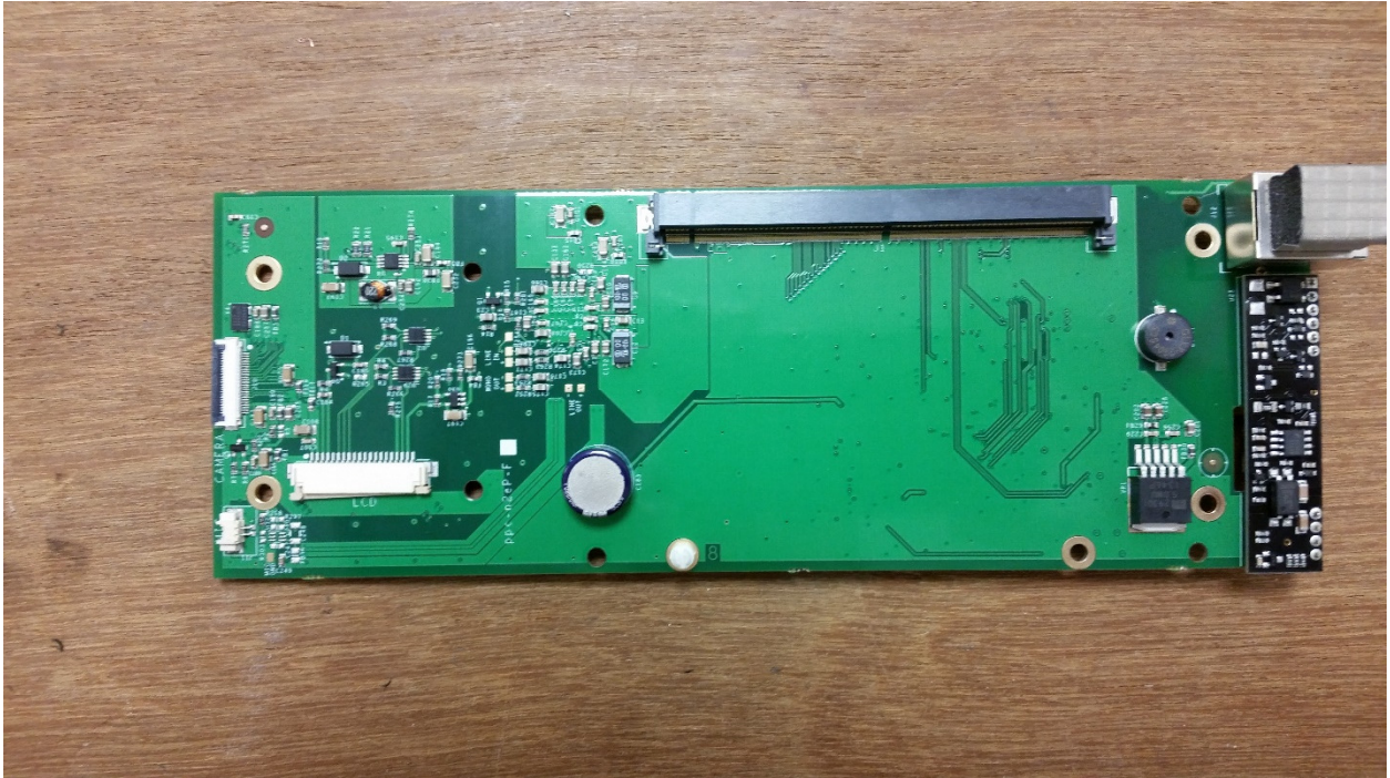
Carrier PCB Top View
