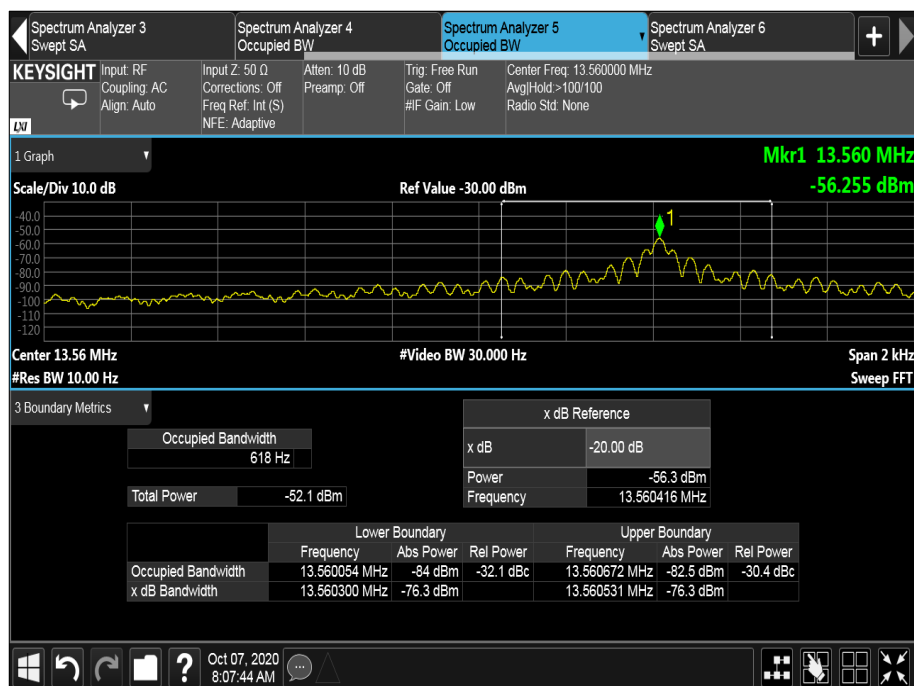
Figure 7 - 99% Occupied Bandwidth
