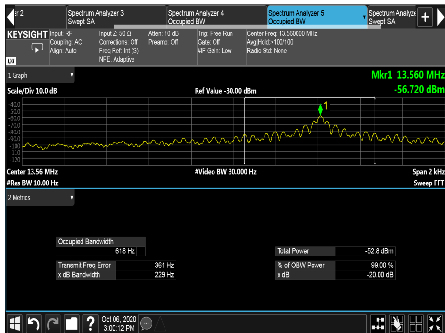
Figure 6 - 20 dB Bandwidth
