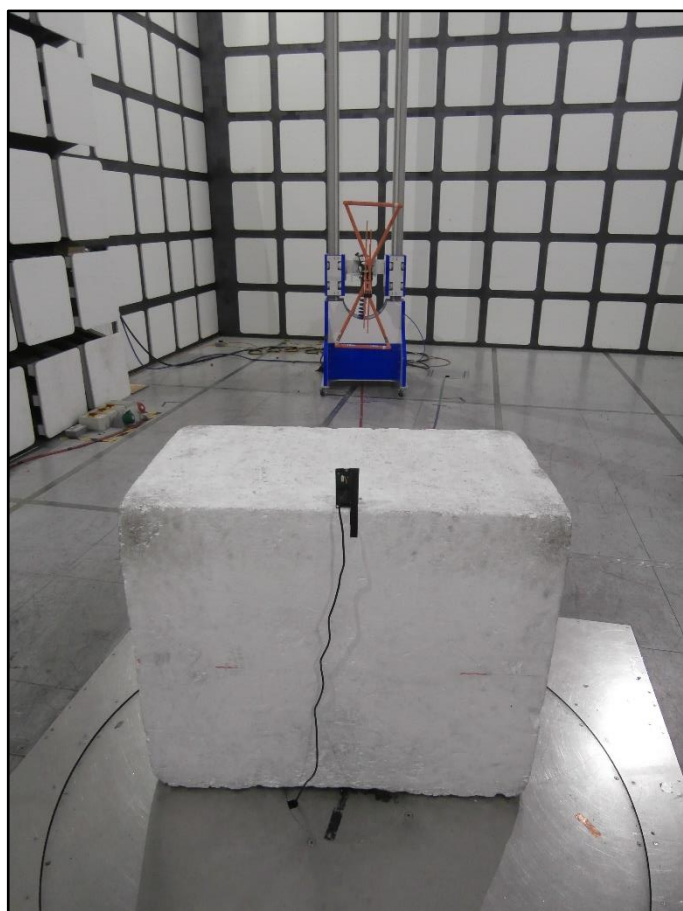
Figure 15 – Test Setup - 30 MHz to 1 GHz
