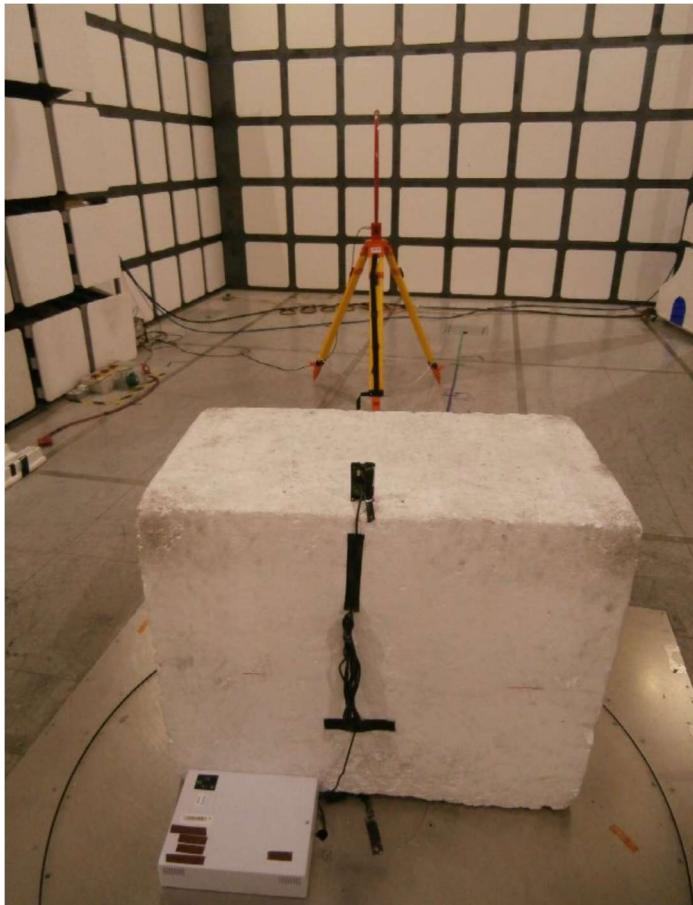
Test Setup - 9 kHz to 30 MHz - Edge On
