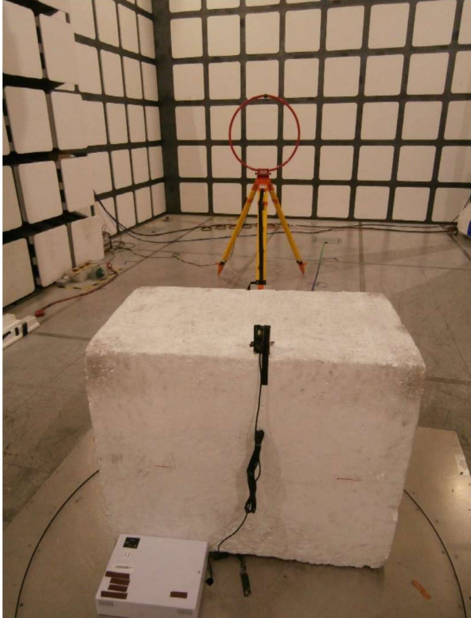
Test Setup - 9 kHz to 30 MHz - Face On
