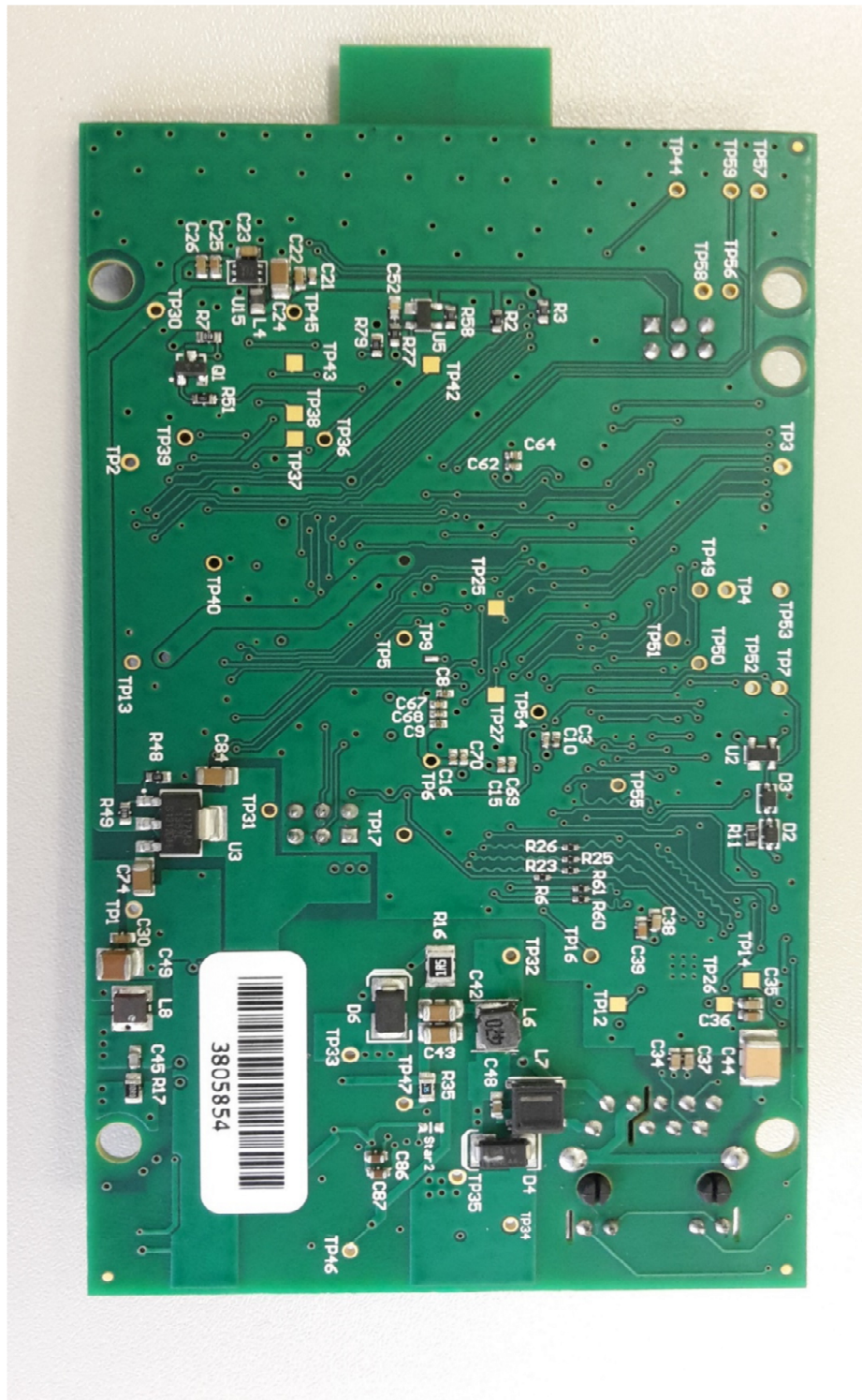
Photo 2 - Track side of PCA
