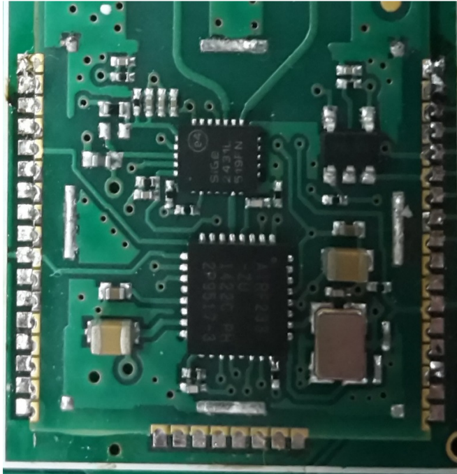
Photo 4b – Bottom of module with shield removed
