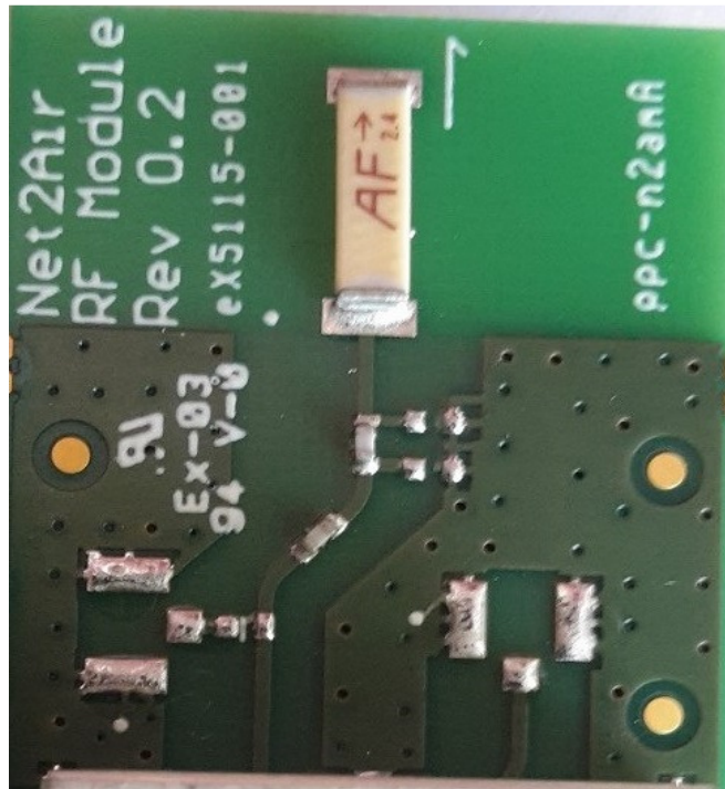
Photo 4a Top of module
