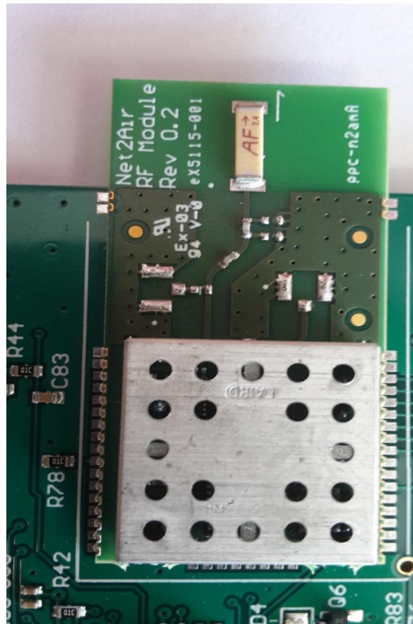
Photo 3 Module with EMC shield
