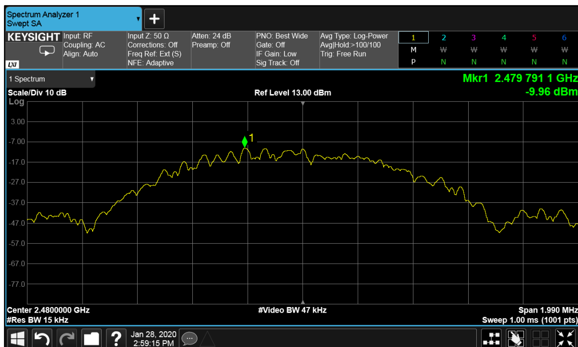
Figure 31 – 2480.0 MHz
