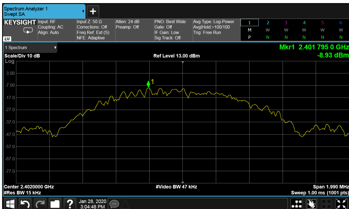
Figure 29 – 2402.0 MHz
