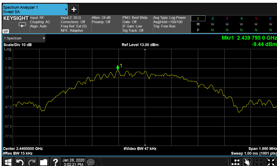
Figure 30 – 2440.0 MHz
