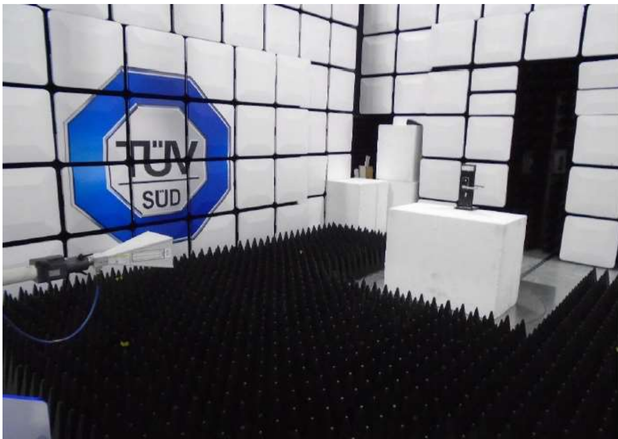
Figure 2– Test Setup Photos 1GHz to 8GHz
