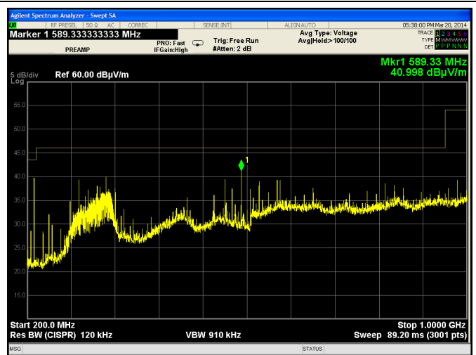
200-1000 MHz – Vertical
