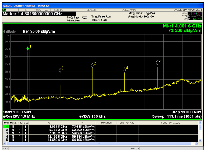
Channel 7 – EUT Vertical – Horizontal Vertical
