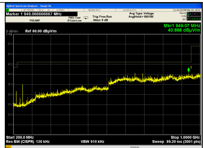
200-1000 MHz Horizontal
