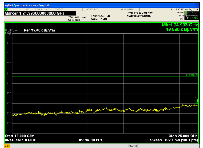
18-25 GHz - Average
