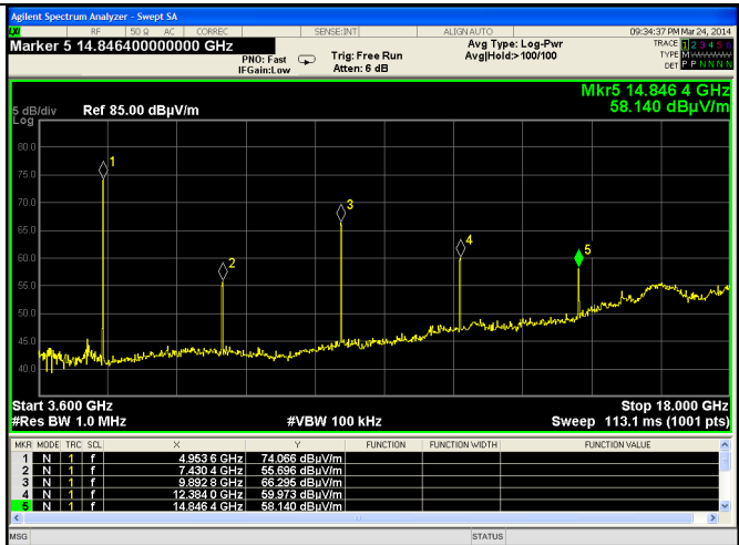
Channel 7 – EUT Cradle – Horizontal Vertical
