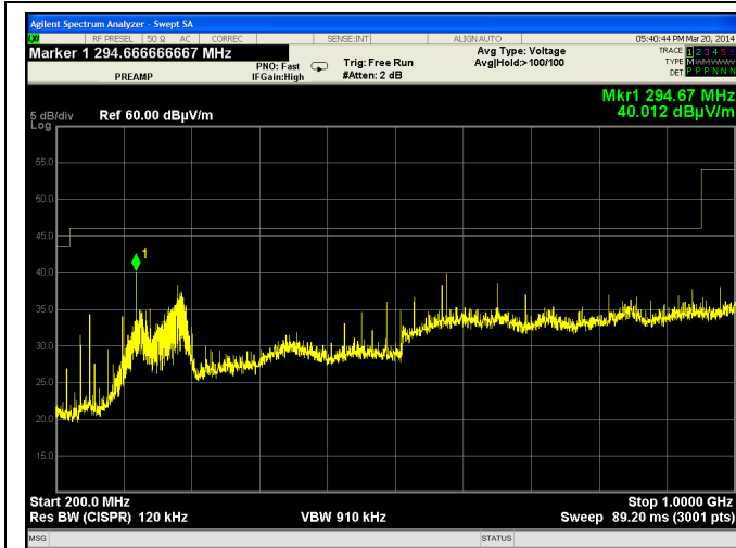
200-1000 MHz – Horizontal
