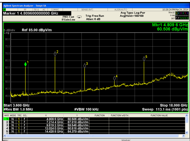
Channel 0 – EUT Flat – Horizontal Vertical
