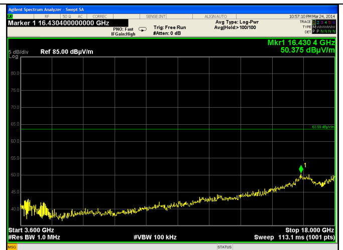
3.6-18 GHz – Average - Horizontal
