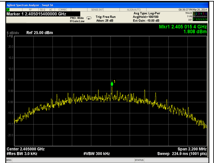
Peak Power Spectral Density
