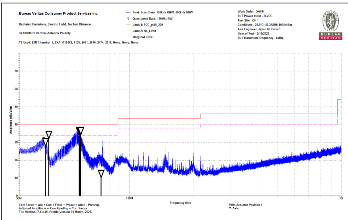
30-1000MHz Vertical Plot
