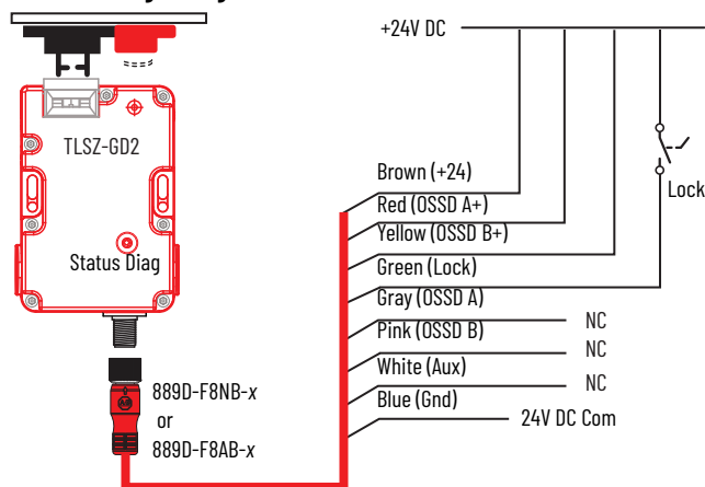
Figure 16 - Commissioning Wiring
