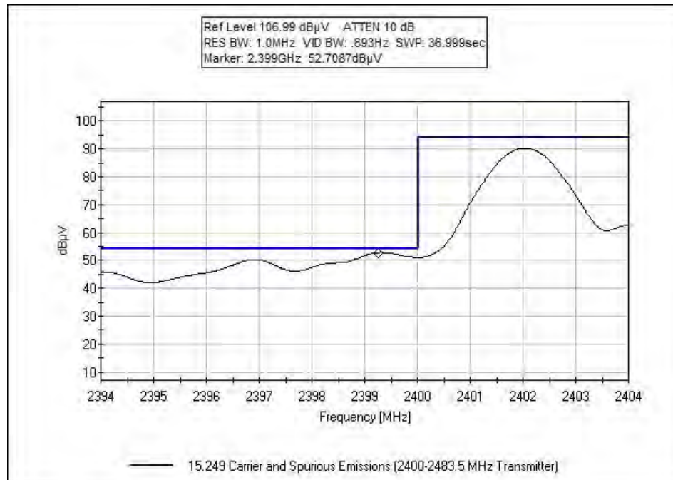
Low Frequency- Average, 3754
