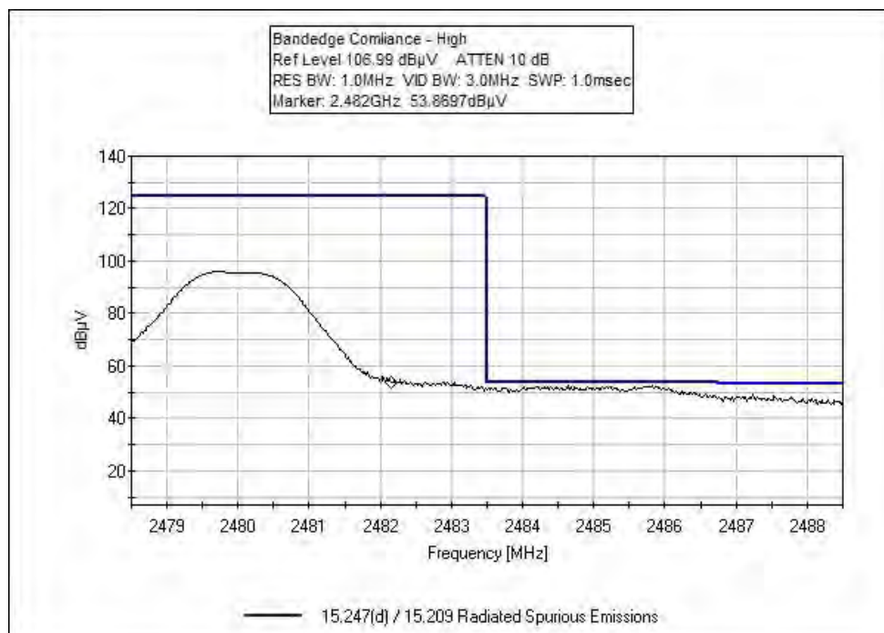
High Frequency- Peak, 3764
