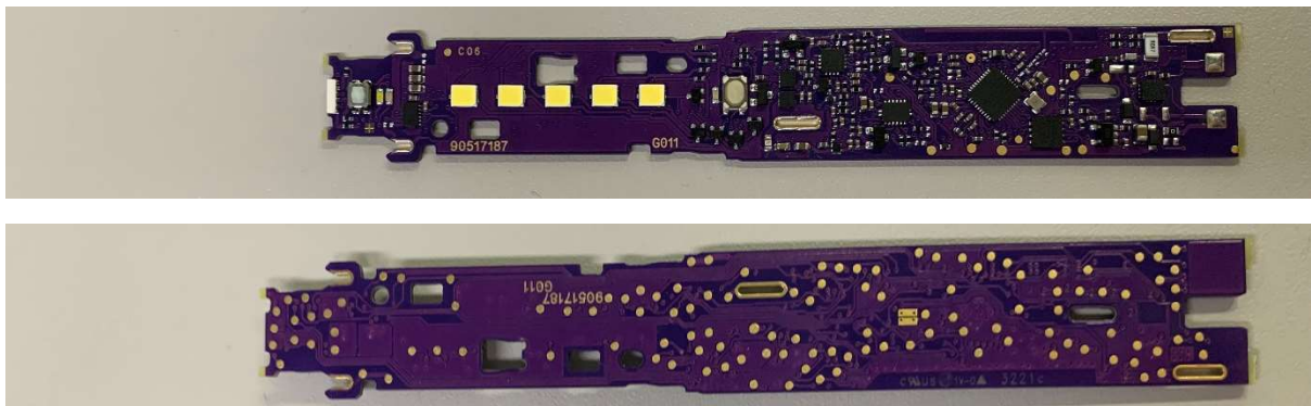
PCB View (top and bottom)
