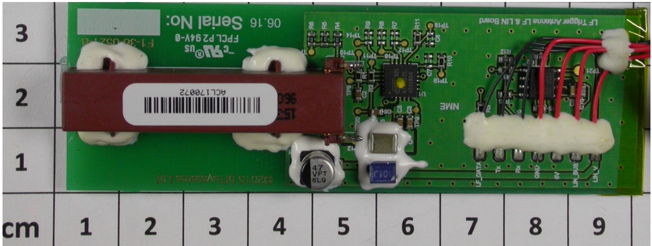
PCB 1:
