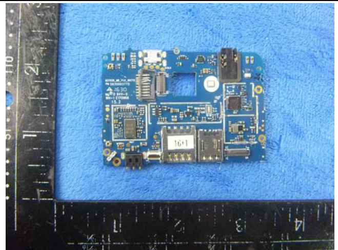
Mainboard witout sheilding – Rear View
