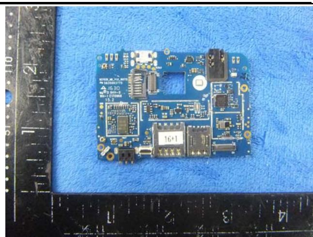
Mainboard witout sheilding – Rear View
