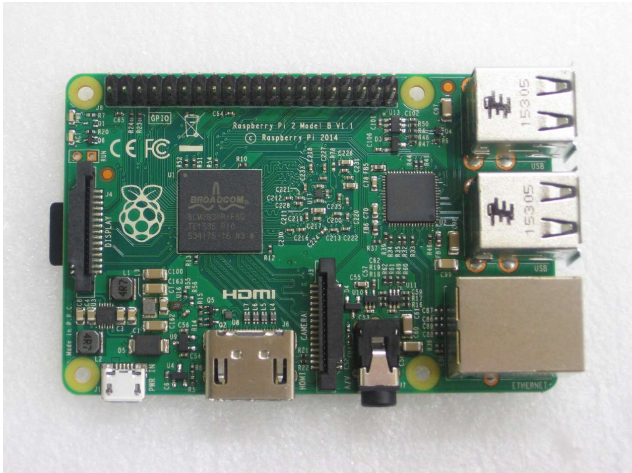
EUT, Main board with daughter board removed – top view
