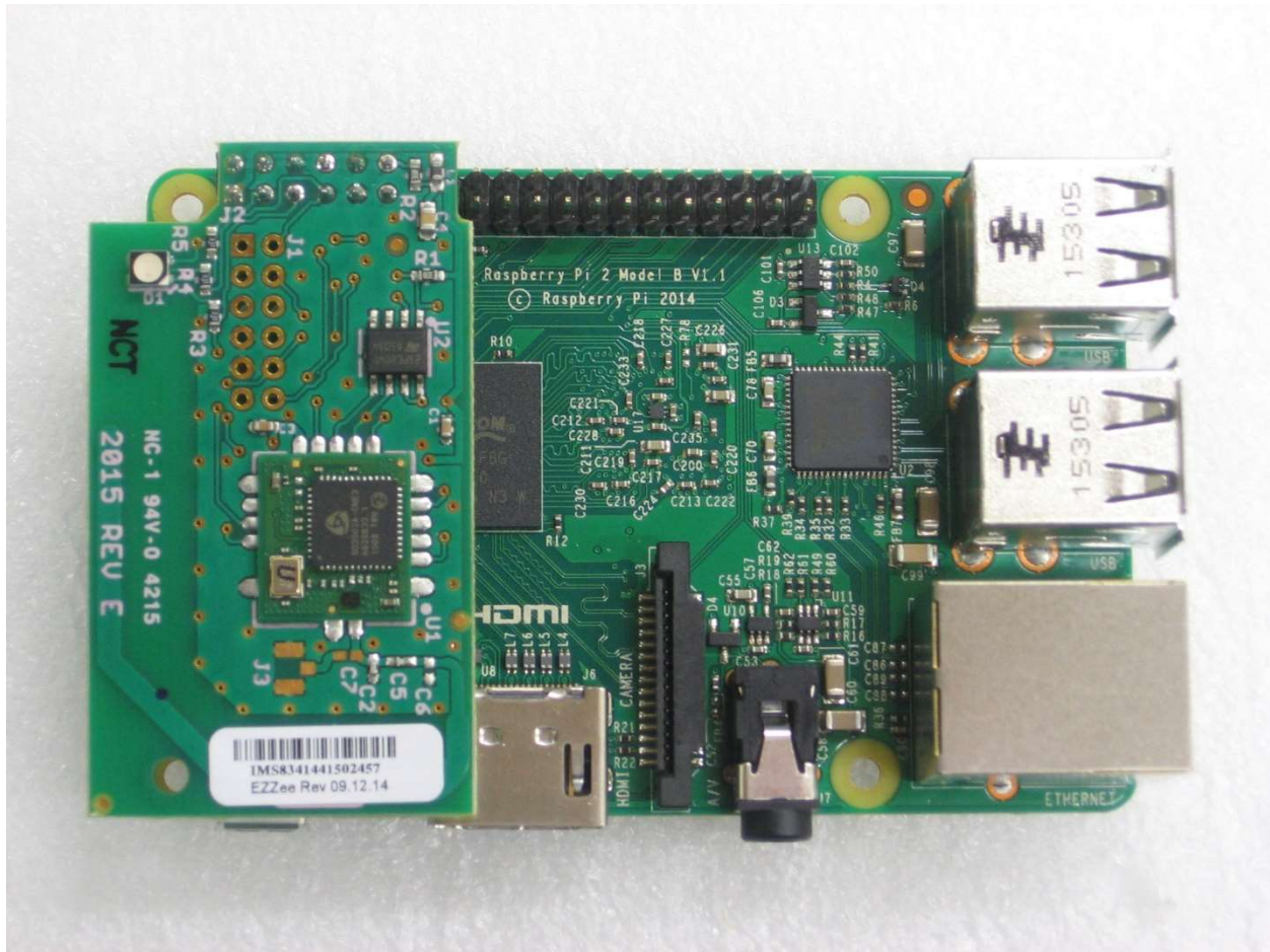
EUT, Main board with daughter board
