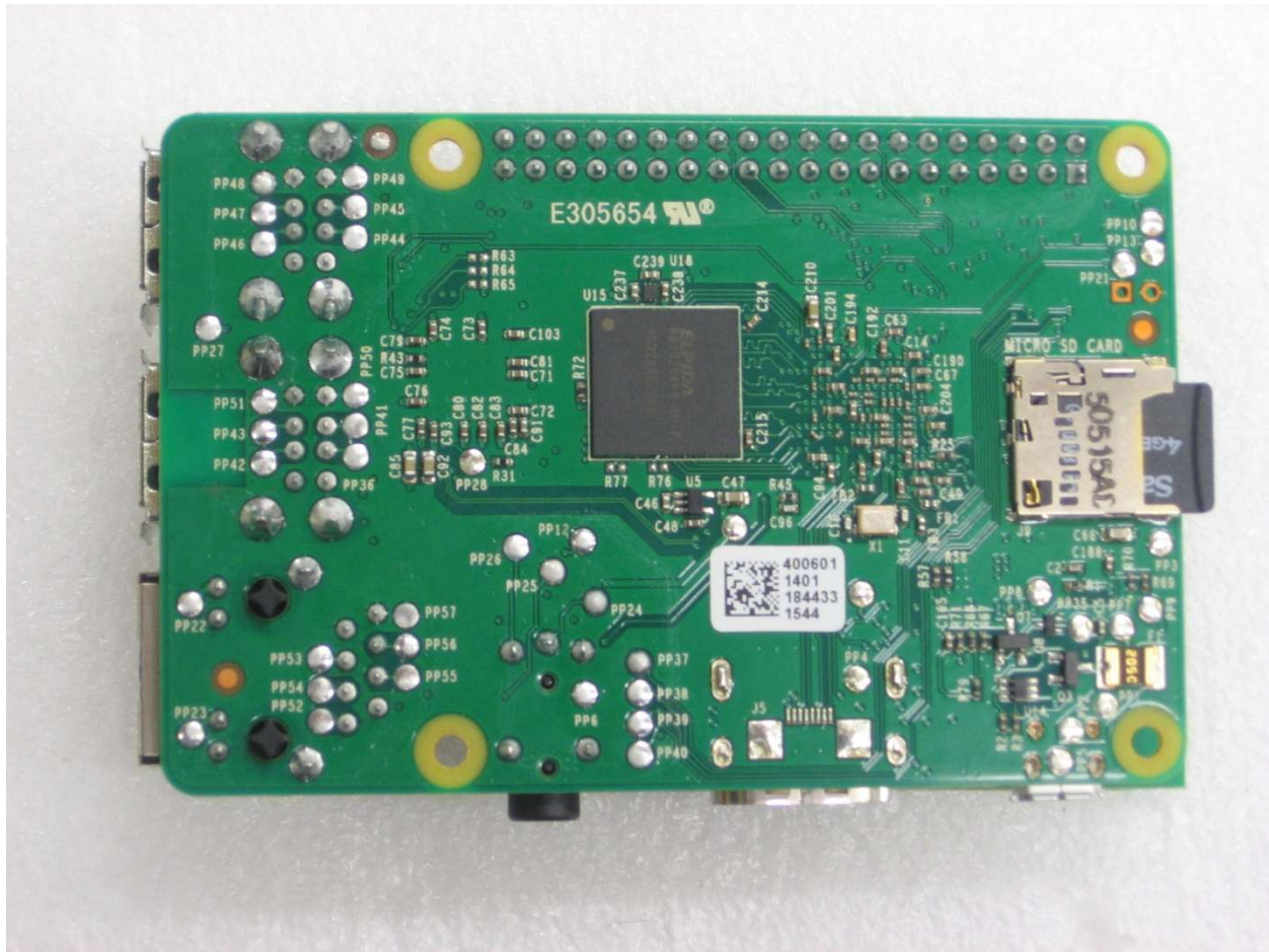
EUT, Main board – bottom view
