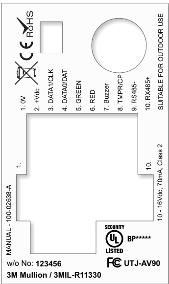
VIEW - REVERSE ▲ standard label format and layout
