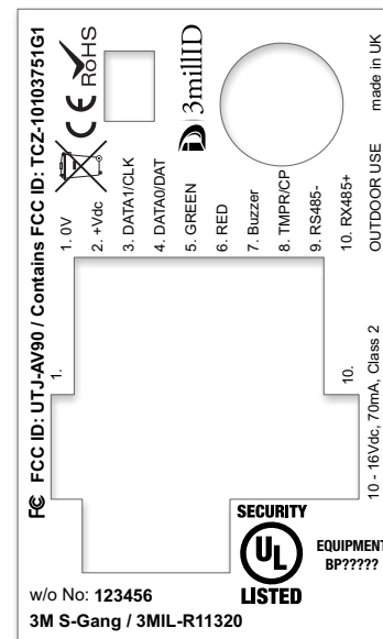
VIEW - REVERSE ▲ standard label format and layout (scale 1:1)
