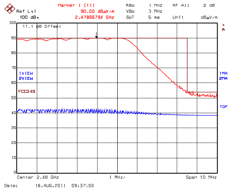
Plot 5.6.4.8. Band-Edge RF Radiated Emissions @ 3 m, Hopping Mode High End of Frequency Band, 2480 MHz, Rx Antenna Orientation: Vertical
