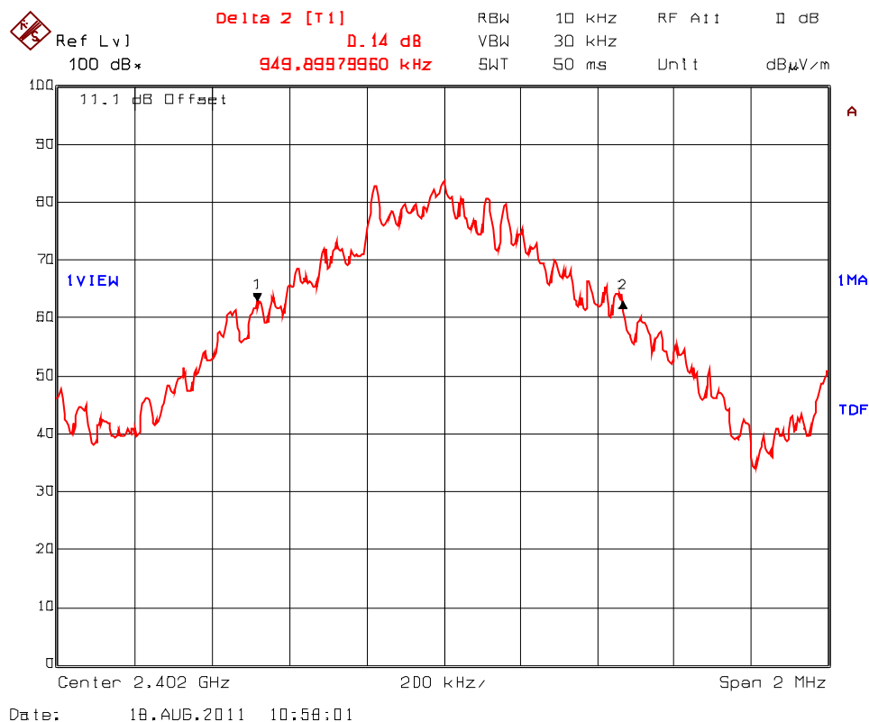
Plot 5.5.4.1. 20 dB Bandwidth, PRBS9 data Test Frequency: 2402 MHz
