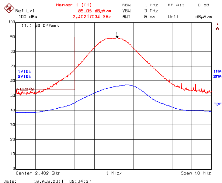
Plot 5.6.4.2. Band-Edge RF Radiated Emissions @ 3 m, Hopping Mode Low End of Frequency Band, 2402 MHz, Rx Antenna Orientation: Horizontal
