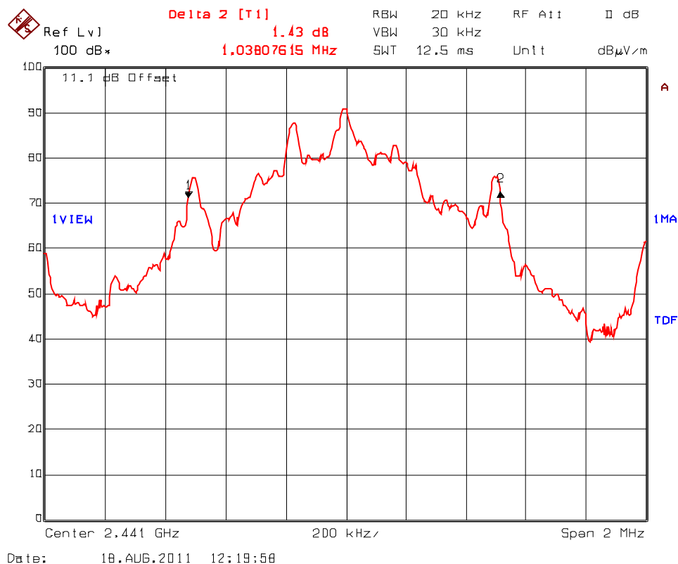
Plot 5.5.4.5. 20 dB Bandwidth, Sequence 101010... data Test Frequency: 2441 MHz
