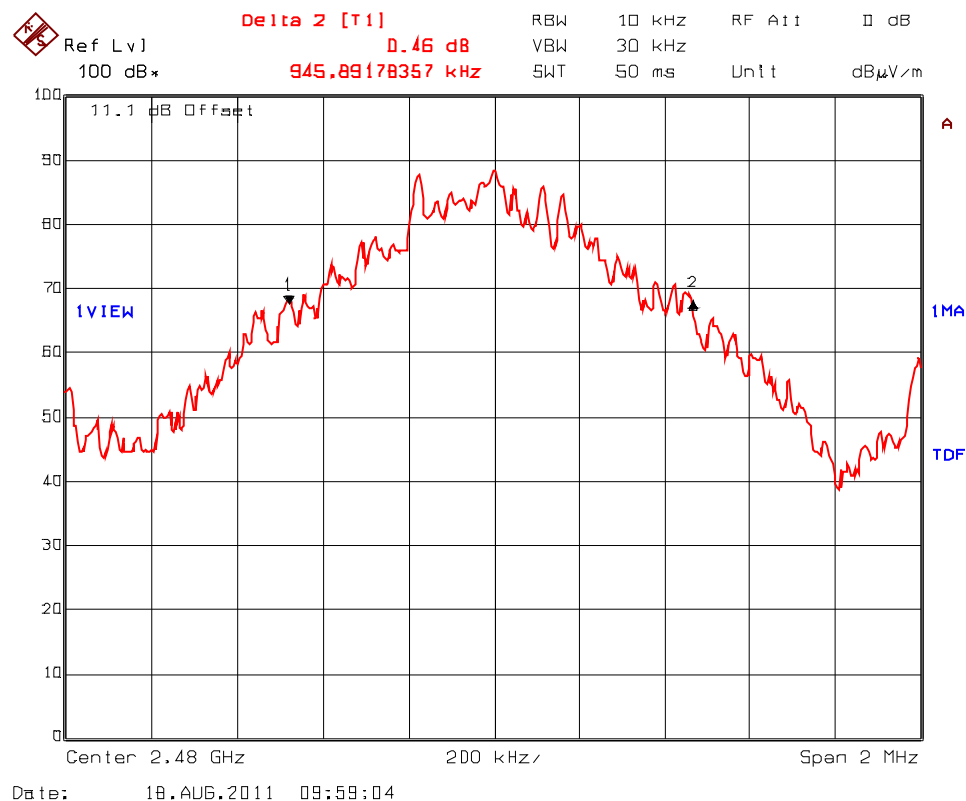
Plot 5.5.4.3. 20 dB Bandwidth Bandwidth, PRBS9 data Test Frequency: 2480 MHz
