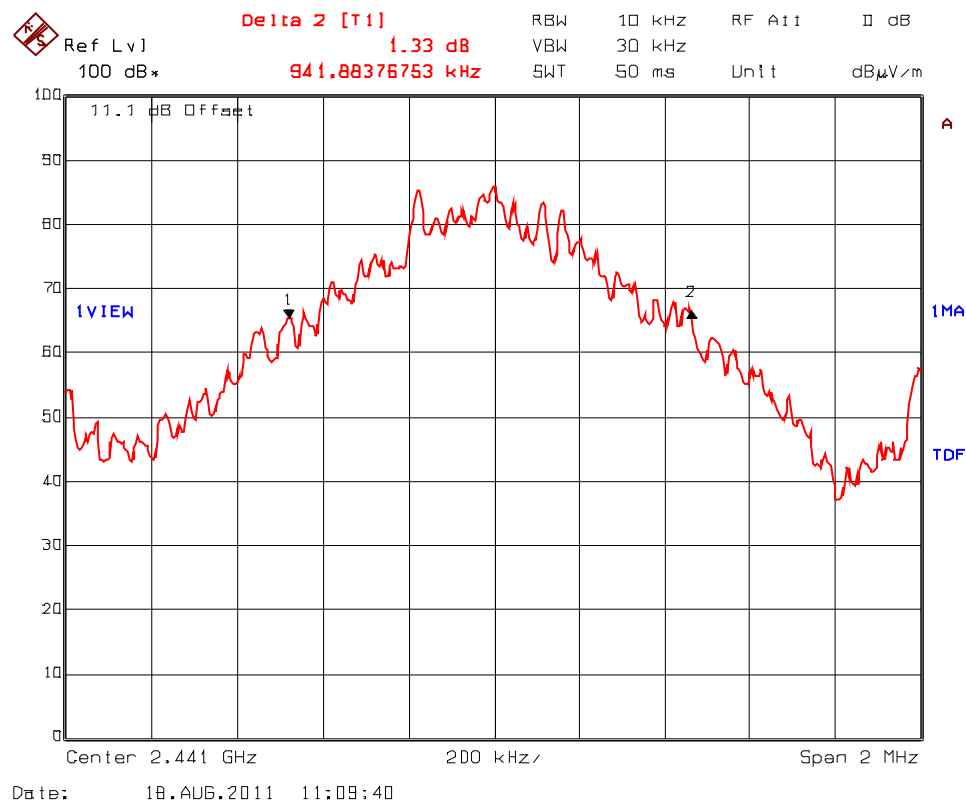
Plot 5.5.4.2. 20 dB Bandwidth, PRBS9 data Test Frequency: 2441 MHz
