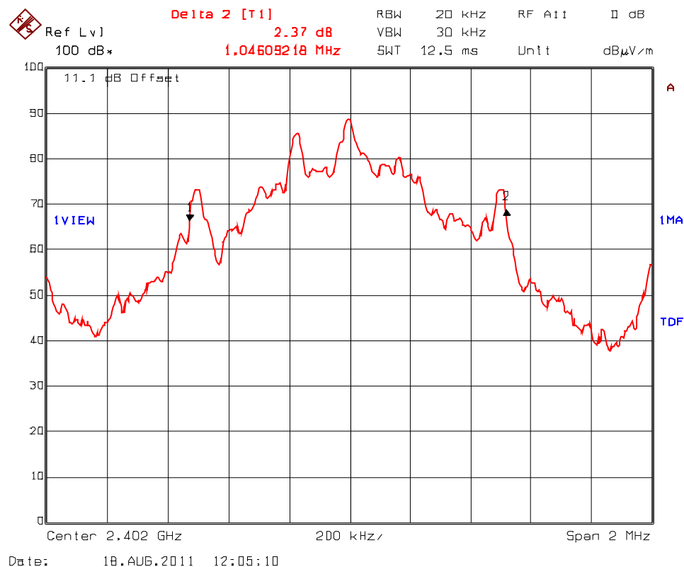
Plot 5.5.4.4. 20 dB Bandwidth, Sequence 101010... data Test Frequency: 2402 MHz
