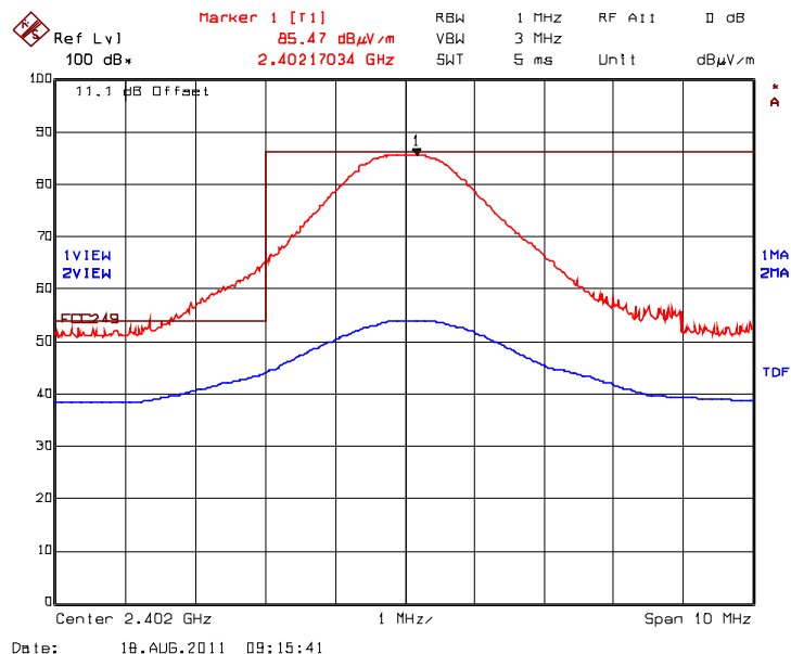
Plot 5.6.4.4. Band-Edge RF Radiated Emissions @ 3 m, Hopping Mode Low End of Frequency Band, 2402 MHz, Rx Antenna Orientation: Vertical
