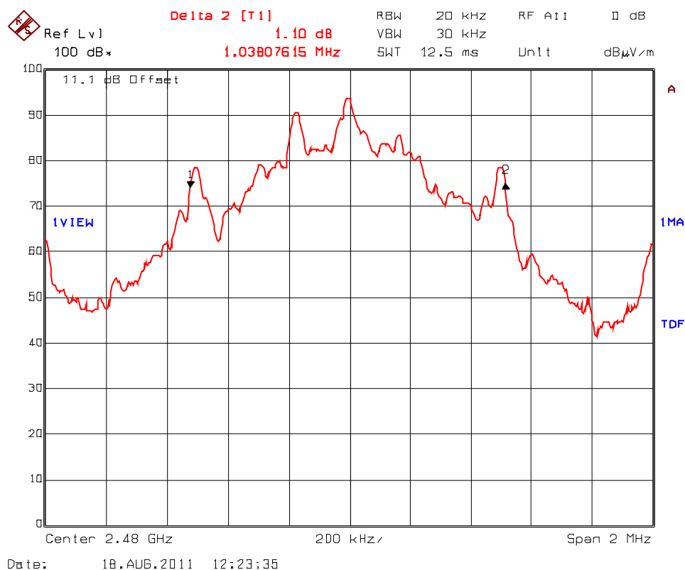
Plot 5.5.4.6. 20 dB Bandwidth Bandwidth, Sequence 101010... data Test Frequency: 2480 MHz
