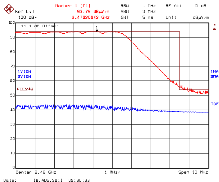
Plot 5.6.4.6. Band-Edge RF Radiated Emissions @ 3 m, Hopping Mode High End of Frequency Band, 2480 MHz, Rx Antenna Orientation: Horizontal
