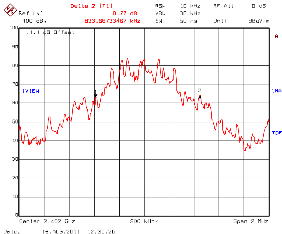
Plot 5.5.4.7. 20 dB Bandwidth, Sequence 1111000011110000... data Test Frequency: 2402 MHz
