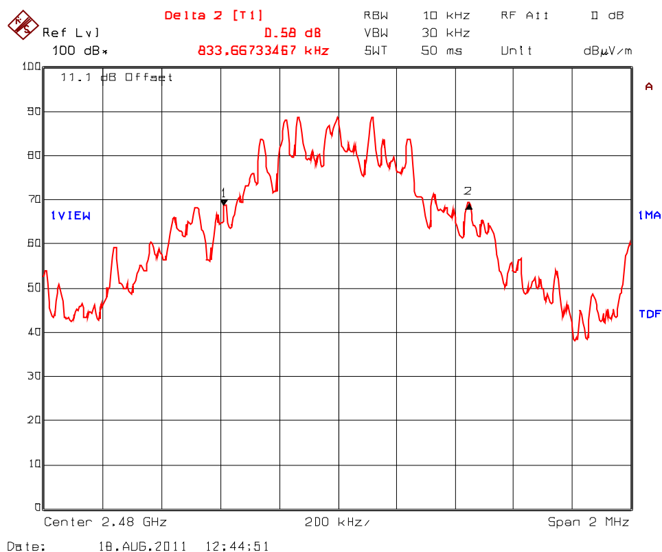
Plot 5.5.4.9. 20 dB Bandwidth Bandwidth, Sequence 1111000011110000... data Test Frequency: 2480 MHz
