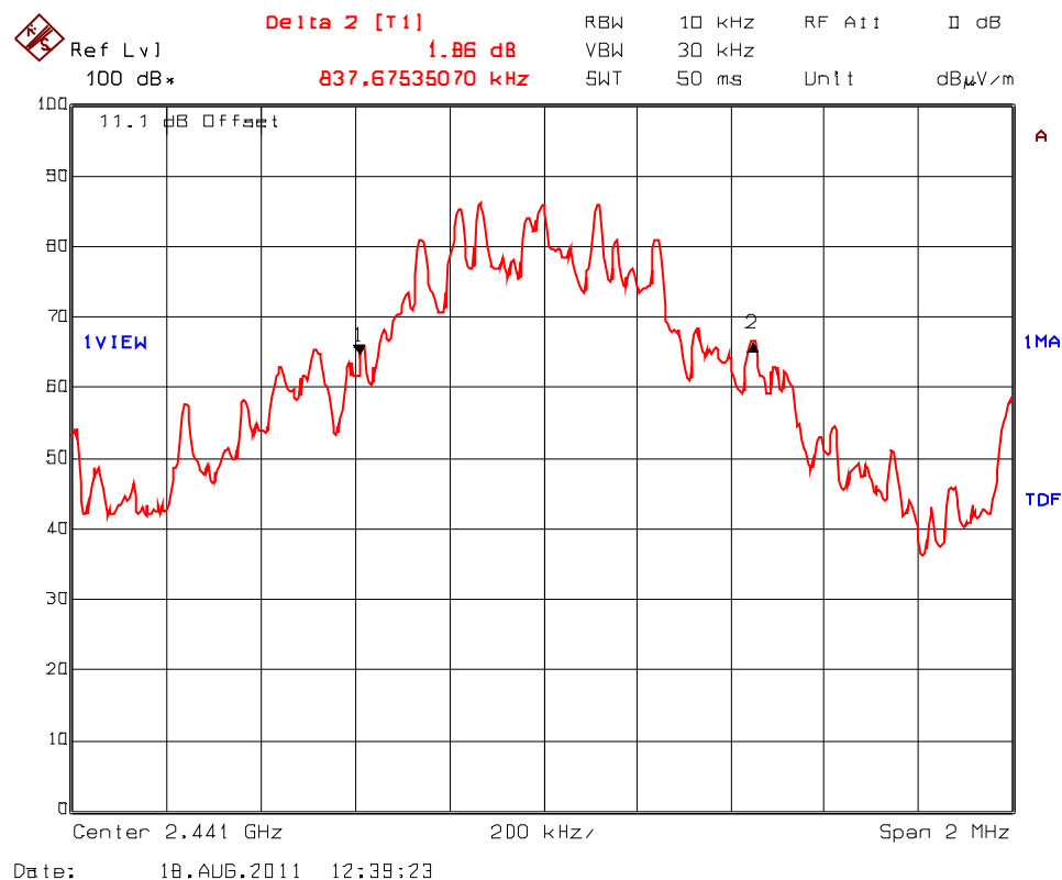
Plot 5.5.4.8. 20 dB Bandwidth, Sequence 1111000011110000... data Test Frequency: 2441 MHz
