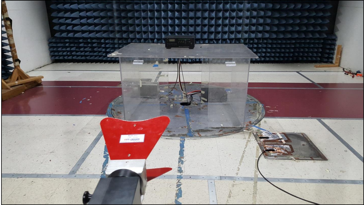
Photograph 5. 97.307(e) Radiated Spurious Emissions for TX Operating Between 30-225 Test Setup (Front View)
