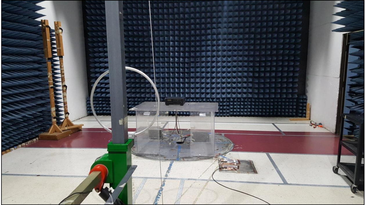
Photograph 3. 97.307(d) Radiated Spurious Emissions for TX Operating Below 30 MHz Test Setup (Front View)
