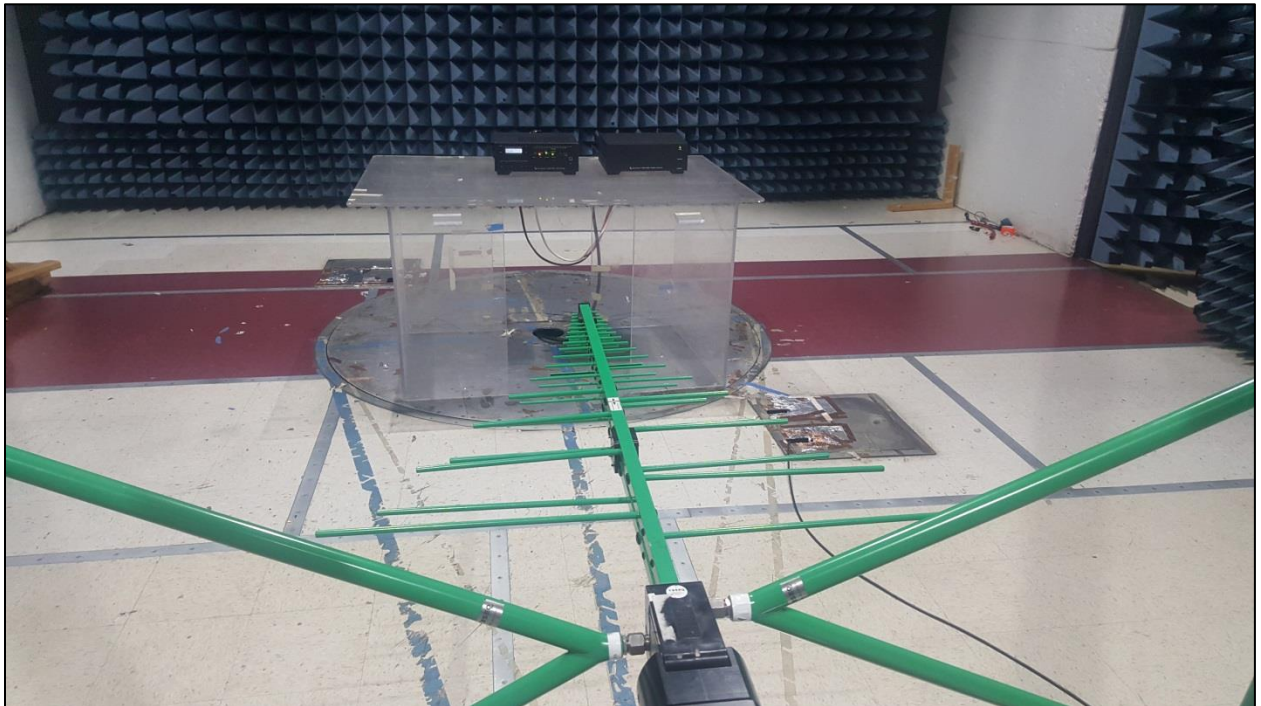
Photograph 4. 97.307(e) Radiated Spurious Emissions for TX Operating Above 30 MHz Test Setup
