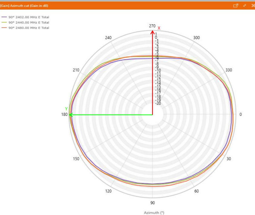
Figure 8.41. Typical 2D Antenna Radiation Patterns - Theta 90° (Front View) Gain (dBi)
