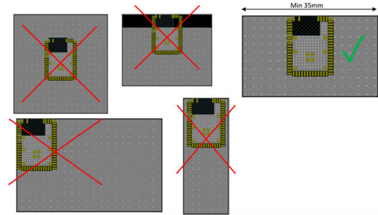
Figure 8.35. Layout Examples
