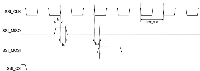
Figure 7.22. Interface Timing Diagram for ULP SSI -- Full Speed Mode
