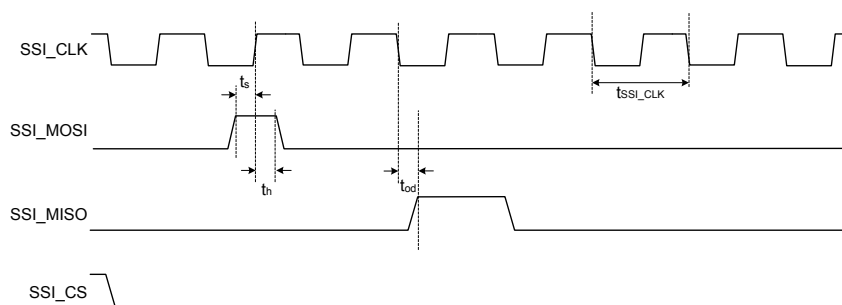
Figure 7.21. Interface Timing Diagram for SSI Secondary Full Speed Mode
