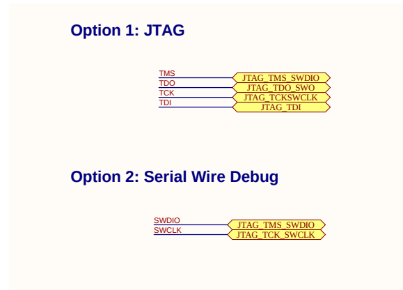
Figure 8.14. JTAG or Serial Wire Debug Interface
