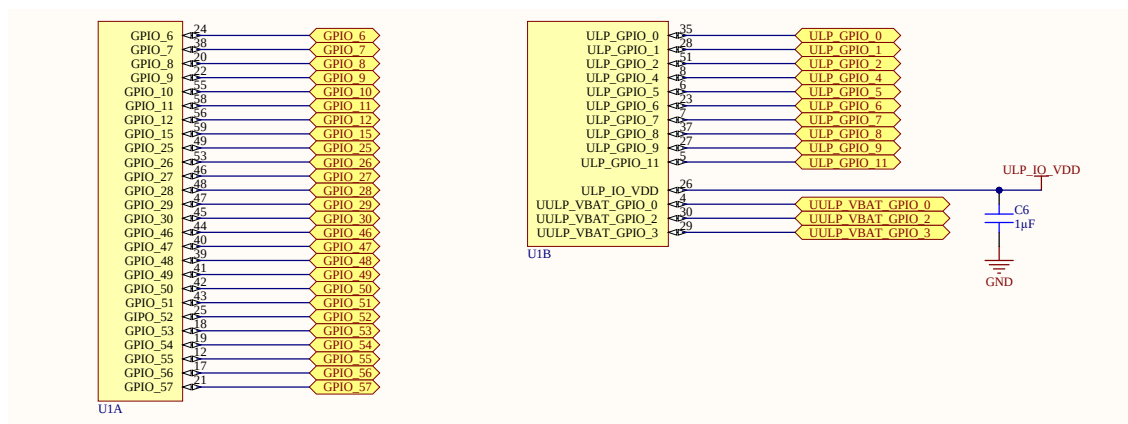
Figure 8.3. GPIO Connection
