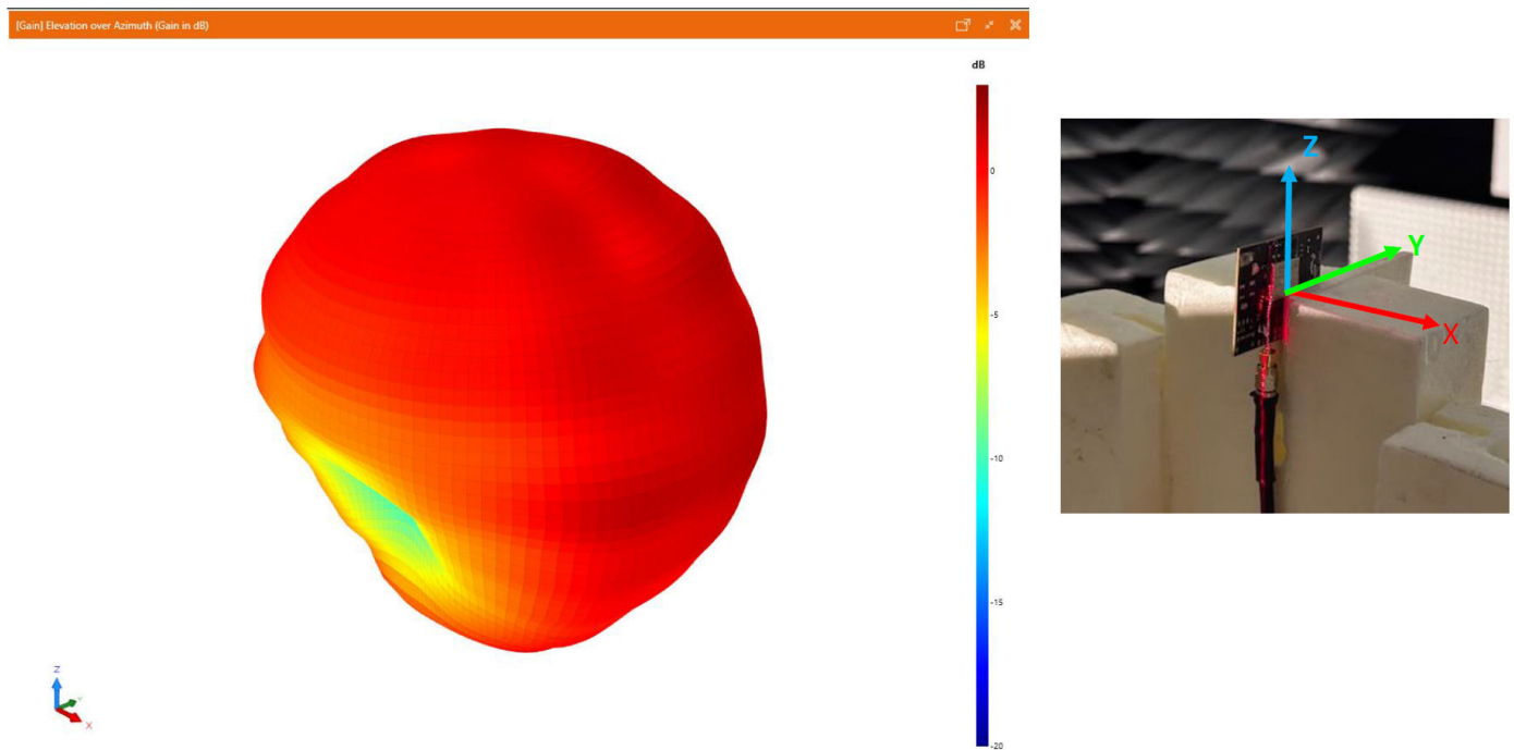
Figure 8.38. 3D Radiation Pattern of the Build-In Antenna
