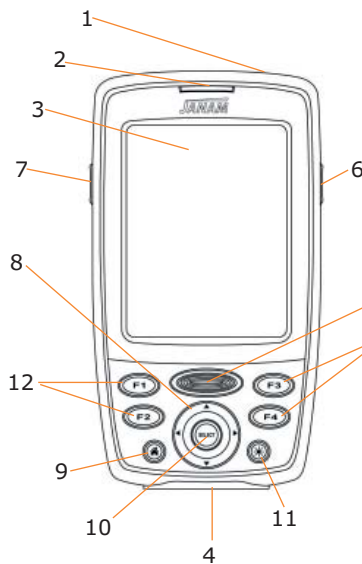
PDA Keypad
