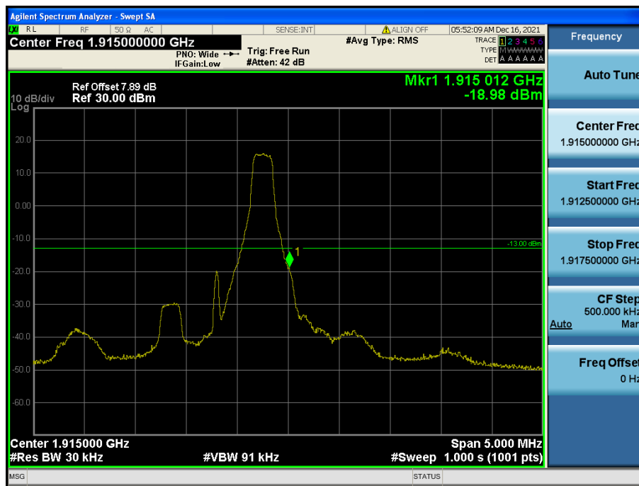
LTE Band 25(2) / 1.4 MHz / 16QAM - RB Size/Offset (1/5)
