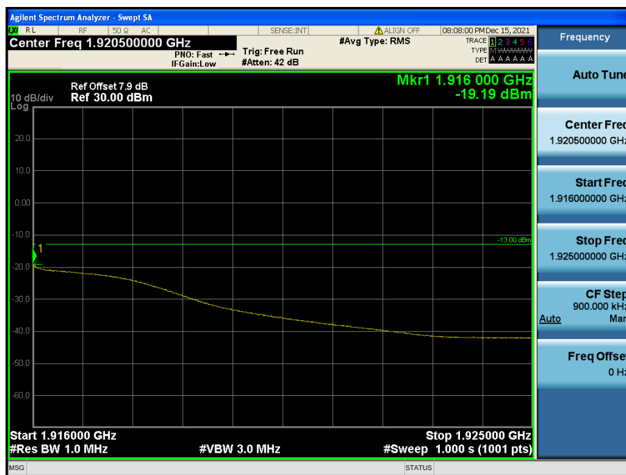
LTE Band 25(2) / 10 MHz / QPSK - RB Size/Offset (25/25)
