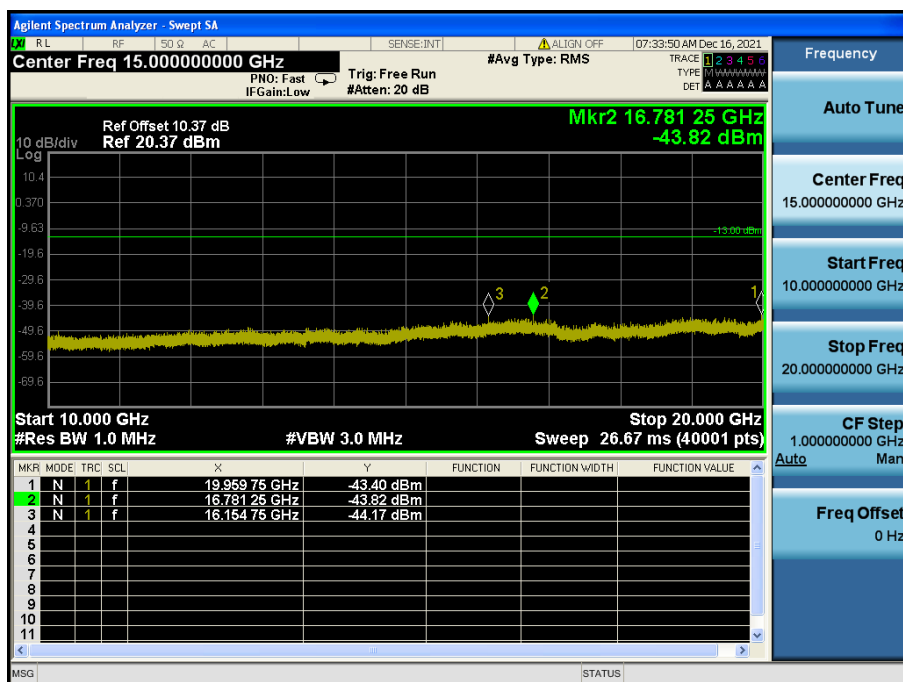
LTE Band 25(2) / 5 MHz / 16QAM - RB Size/Offset (25/0) – High Channel
