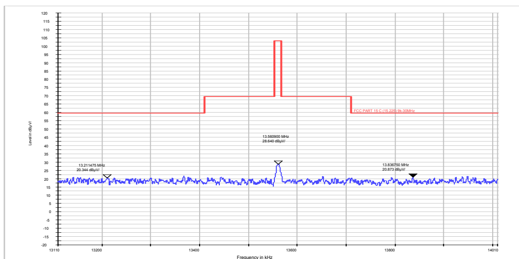
ANT-Horizontal
