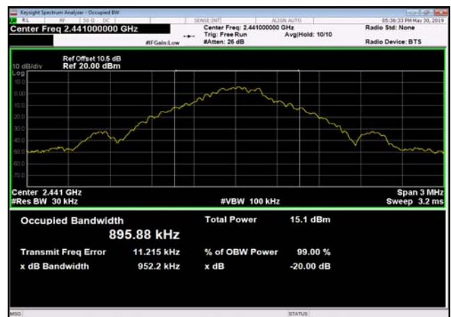
99% Bandwidth: GFSK,2441MHz,DH5
