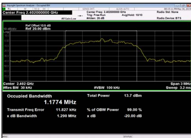
99% Bandwidth: 8DPSK,2402MHz,3DH5
