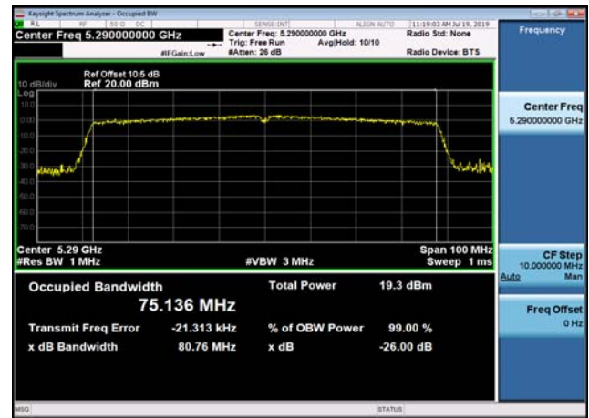
U-NII-2a 99% Bandwidth-802.11ac(80MHz) ,5290MHz
