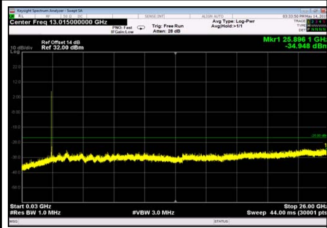
FDD07_MidRange_20MHz_30MHz~26GHz
