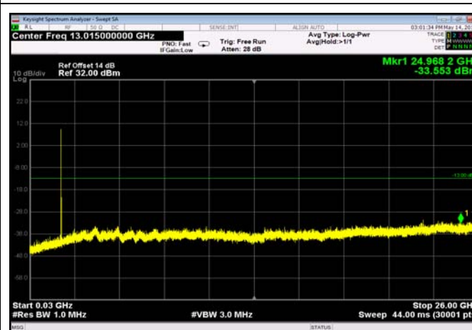
FDD02_LowRange_5MHz_30MHz~26GHz
