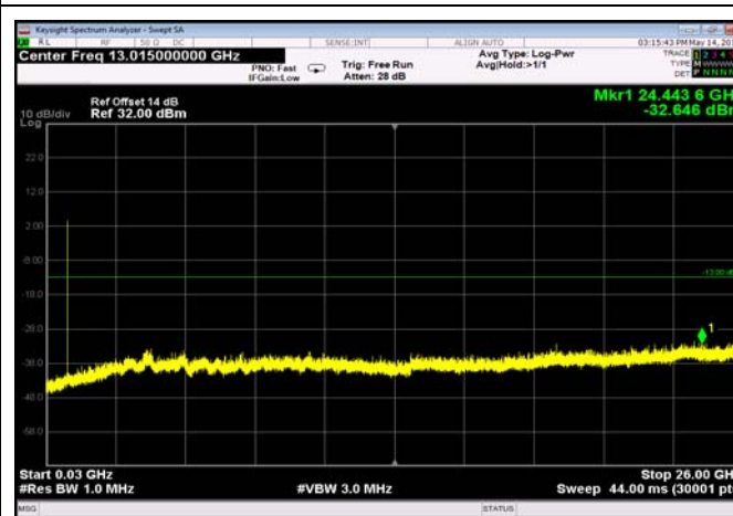
FDD07_HighRange_10MHz_30MHz~26GHz
