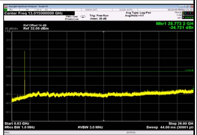
FDD02_MidRange_30MHz_30MHz~26GHz
