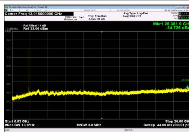
FDD07_LowRange_20MHz_30MHz~26GHz
