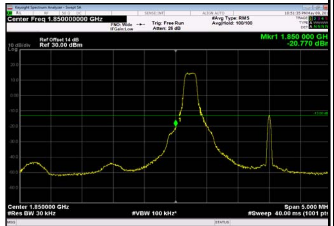
LowRange_FDD02_3MHz_1851.5_fullRB _Low_Q16 16
