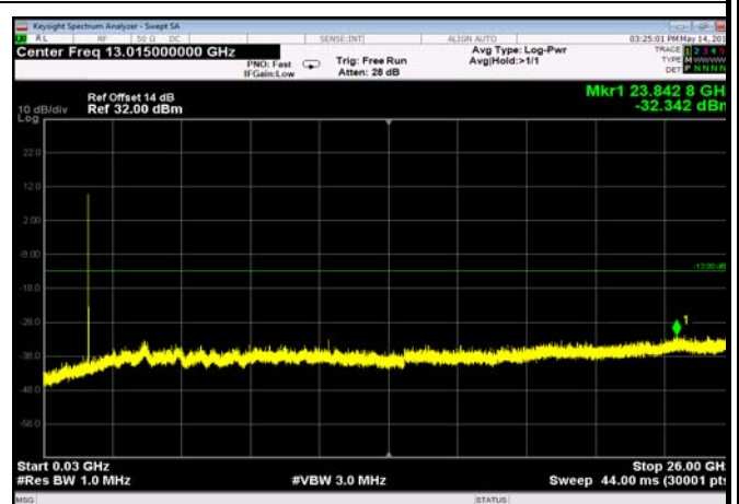
FDD04_LowRange_15MHz_30MHz~26GHz
