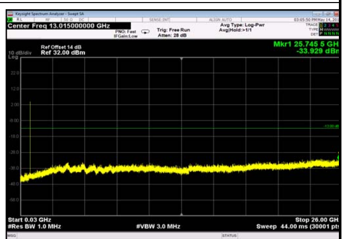
FDD07_HighRange_15MHz_30MHz~26GHz
