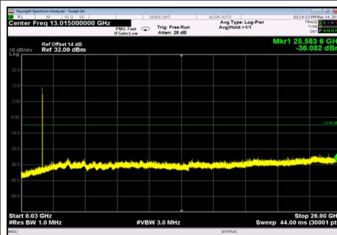
FDD04_HighRange_20MHz_30MHz~26GHz
