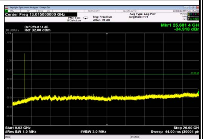
FDD04_MidRange_15MHz_30MHz~26GHz
