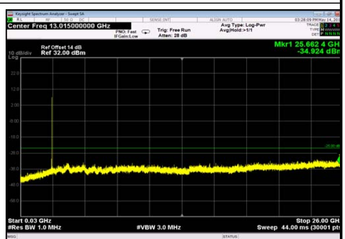
FDD07_HighRange_5MHz_30MHz~26GHz
