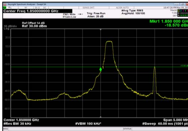
LowRange_FDD02_3MHz_1851.5_fullRB _Low_QPSK 15
