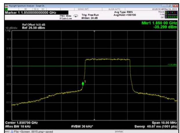
LowRange_FDD02_5MHz_1852.5_OneRB _low_Q16
