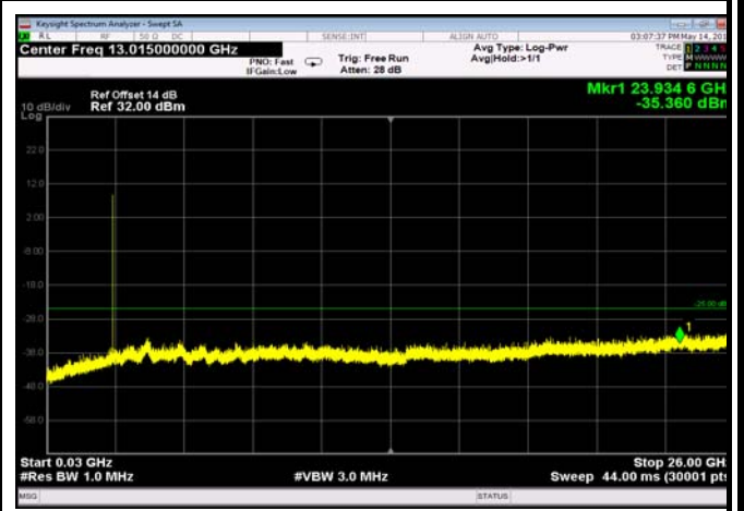
FDD07_MidRange_5MHz_30MHz~26GHz
