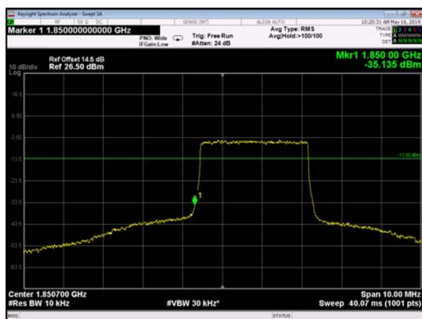
LowRange_FDD02_5MHz_1852.5_OneRB _low_QPSK
