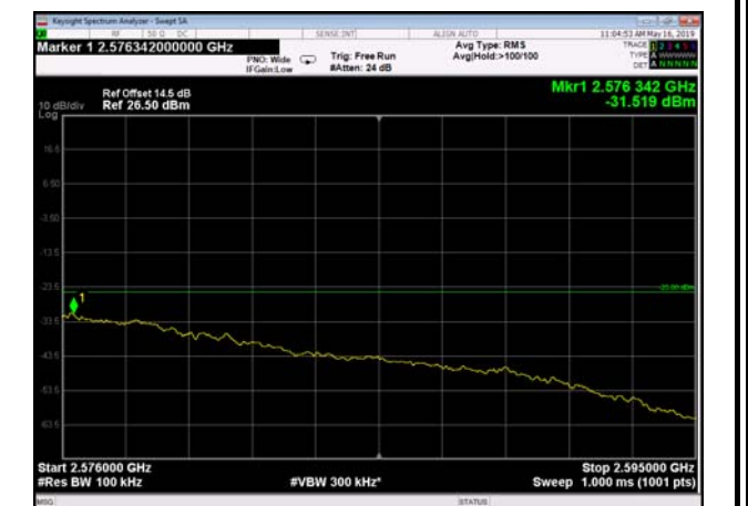
FDD07_15MHz_2562.5_QPSK_fullIRB _ExtraBands_Range_2576~2595 38
