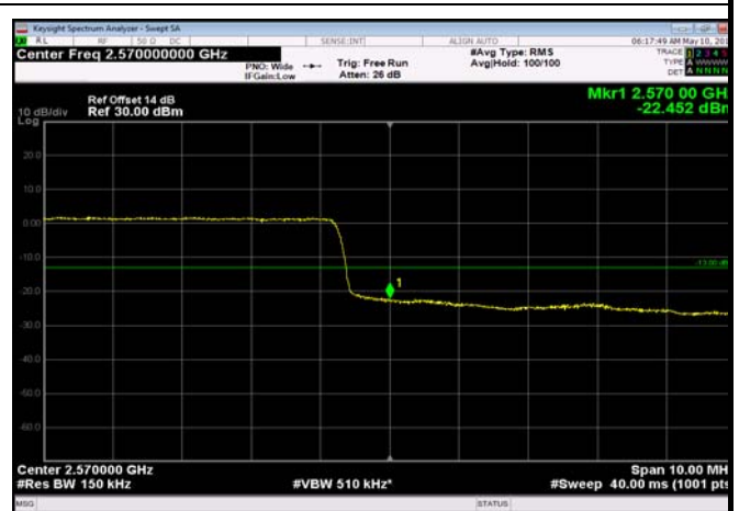
HighRange_FDD07_15MHz_2562.5_fullRB _High_QPSK
