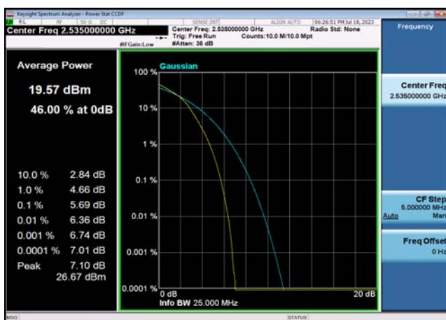
FDD07_MidRange_20MHz_2535_fullIRB _Q16
