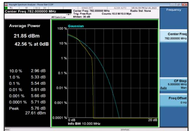
FDD13_LowRange_10MHz_782_OneRB _high_Q16
