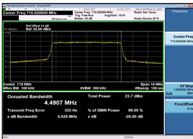
FDD17_MidRange_5_710_QPSK
