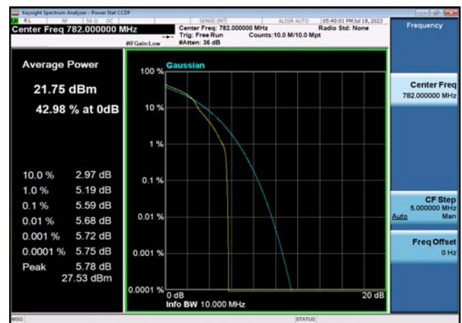
FDD13_MidRange_10MHz_782_OneRB _high_Q16
