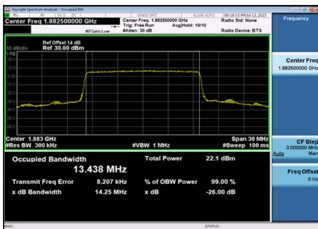
FDD25_MidRange_15_1882.5_QPSK
