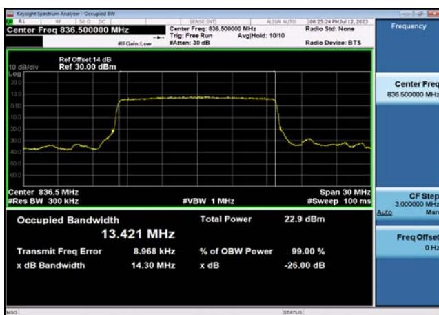
FDD26_(Part 22&RSS-132) _MidRange_15_836.5_QPSK
