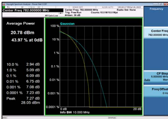
FDD13_LowRange_10MHz_782_fullIRB _Q16
