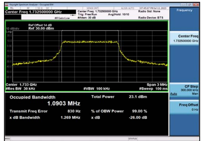
FDD04_MidRange_3_1732.5_Q16
