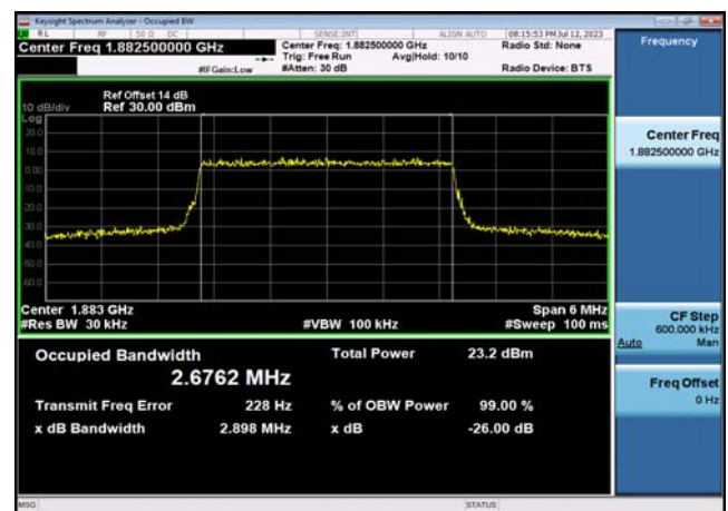
FDD25_MidRange_3_1882.5_Q16
