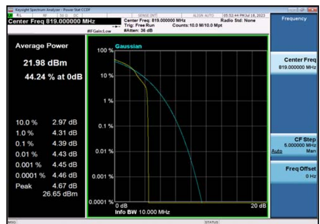
FDD26_Part 90_MidRange_10MHz_819_OneRB _high_Q16
