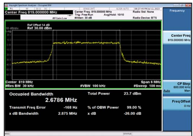
FDD26_Part 90_MidRange_5_819_Q16
