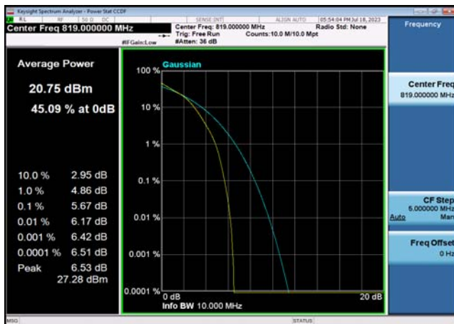
FDD26_Part 90_LowRange_10MHz_819_fullIRB _Q16
