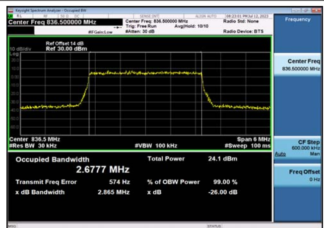
FDD26_(Part 22&RSS-132) _MidRange_3_836.5_Q16
