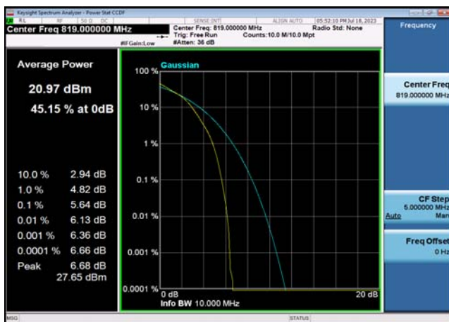
FDD26_Part 90_MidRange_10MHz_819_fullIRB _Q16
