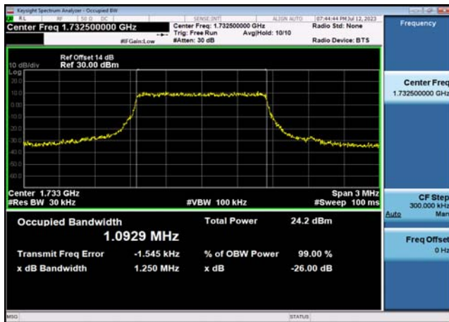
FDD04_MidRange_3_1732.5_QPSK
