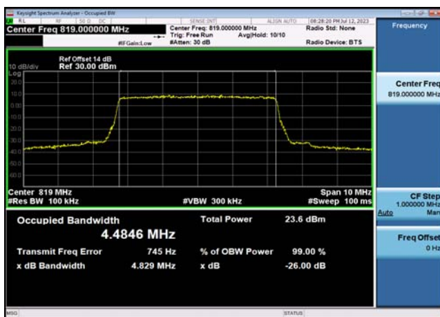
FDD26_Part 90_MidRange_5_819_QPSK
