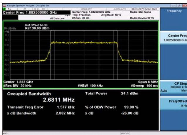
FDD25_MidRange_3_1882.5_QPSK
