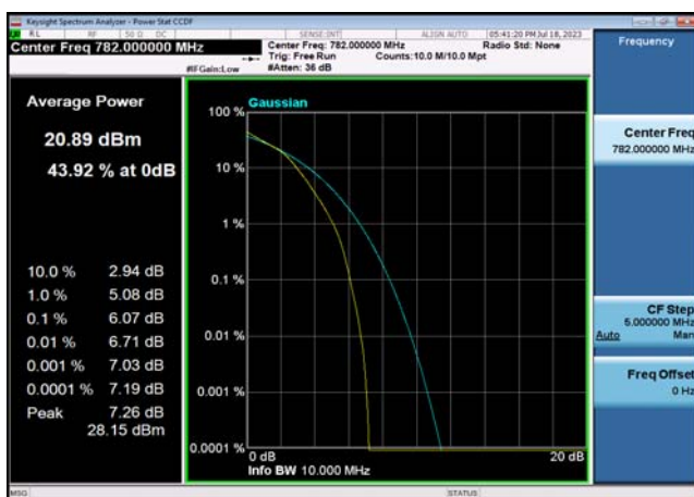
FDD13_MidRange_10MHz_782_fullIRB _Q16
