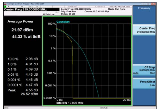
FDD26_Part 90_LowRange_10MHz_819_OneRB _high_Q16
