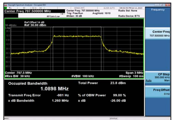
FDD12_MidRange_1.4_707.5_Q16
