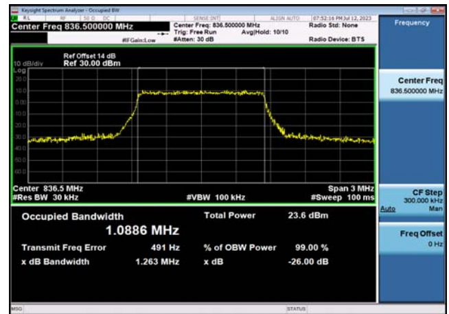
FDD05_MidRange_3_836.5_Q16
