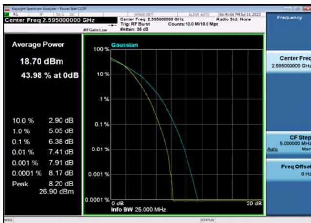
TDD38_MidRange_20MHz_2595_fullIRB _Q16
