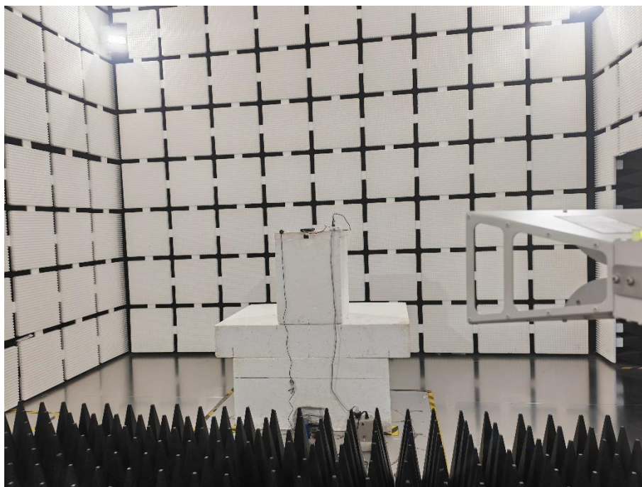
RSE-Above 1GHz-RF
